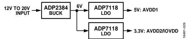
Figure 77. Power Supply Configuration
