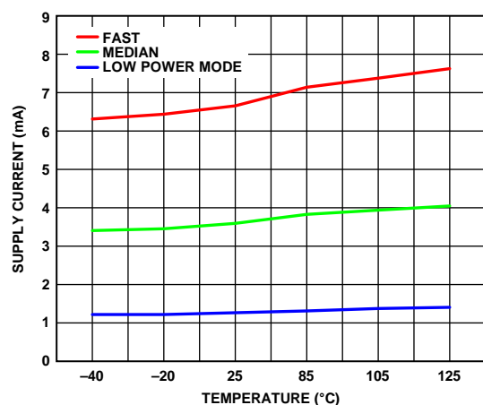
Figure 48. Supply Current vs. Temperature, AVDD1
