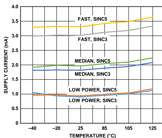
Figure 50. Supply Current vs. Temperature, IOVDD, Sinc3 and Sinc5 Filter
