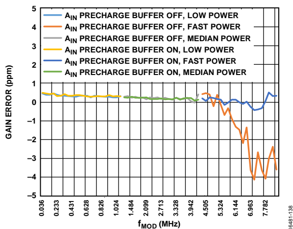
Figure 36. Gain Error vs. f_{MOD}
