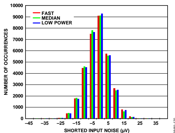
Figure 19. Shorted Input Noise, Sinc5 Filter, Three Power Modes, N = 32,768
