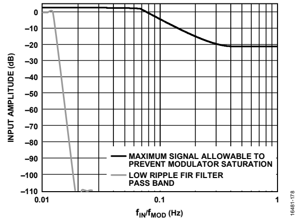
Figure 74. Modulator Saturation Area
