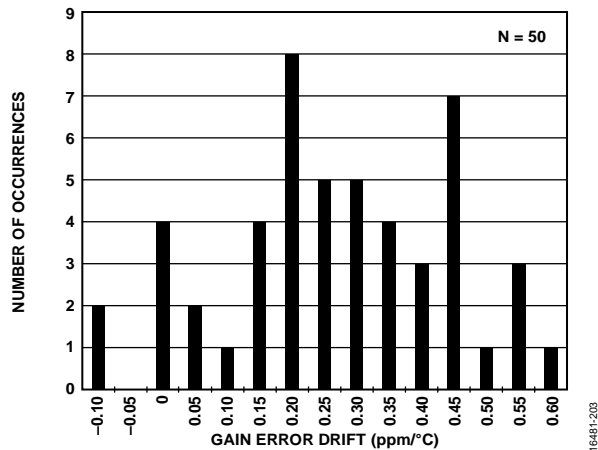
Figure 35. Gain Error Drift Reference Buffers Off
