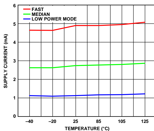
Figure 49. Supply Current vs. Temperature, AVDD2
