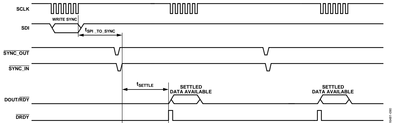
Figure 91. One Shot Conversion Mode, \overline{\text{SYNC\_IN}} Pulse Initiated by a Register Write
