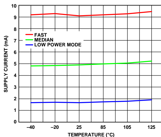
Figure 51. Supply Current vs. Temperature, IOVDD, Low Ripple FIR Filter
