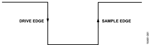
Figure 82. SPI Mode 3
