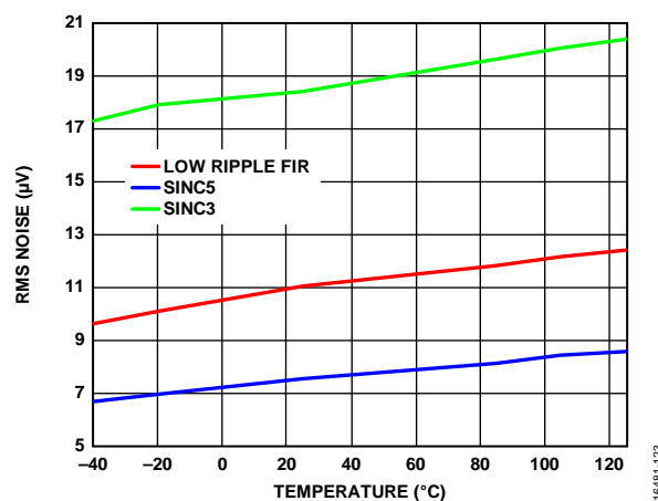
Figure 21. RMS Noise vs. Temperature, Three Filter Types, Fast Mode
