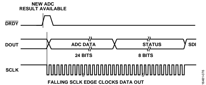
Figure 78. PIN Mode Data Output Format (This Figure Does Not Show the CS Signal)
