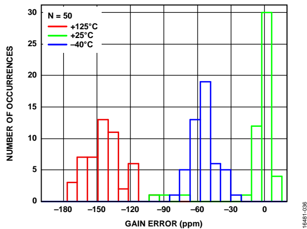
Figure 34. Gain Error Distribution, Reference Buffers On
