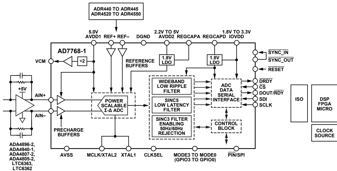
Figure 60. AD7768-1 Top Level Core Signal Chain and Control
