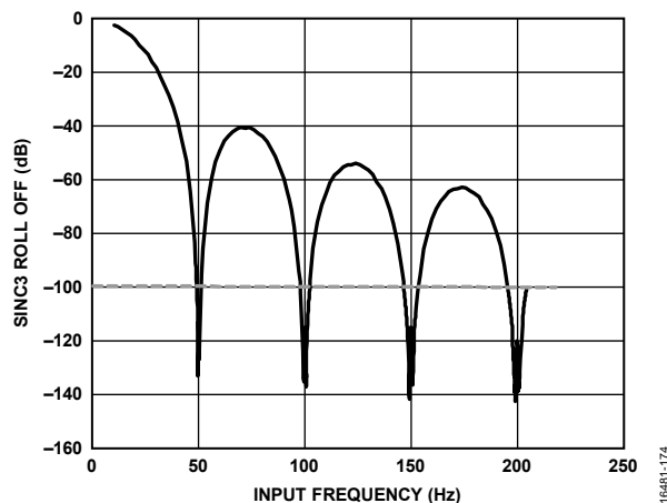
Figure 70. Sinc3 Filter Frequency Response Showing 50 Hz Rejection, 50 Hz ODR, \times 163,840 Decimation
