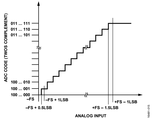
Figure 59. ADC Ideal Transfer Functions (FS is Full-Scale)
