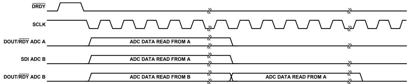
Figure 80. Data Output Format When Devices Daisy-Chained ( \overline{\text{PIN}} Control Mode Only)
