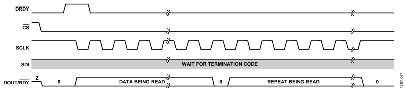
Figure 88. Continuous ADC Read Data Format with \overline{\text{RDY}} Function Disabled
