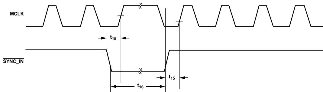
Figure 7. Synchronous \overline{\text{SYNC\_IN}} Pulse
