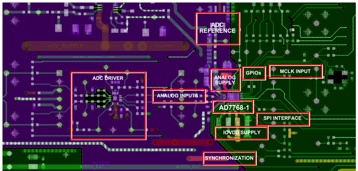
Figure 97. Subsystem Layout
