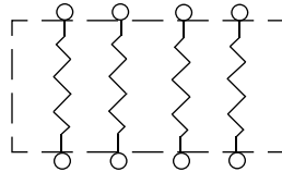
NRSNA4I4/Ø4I NRSNA6I/Ø6I & NRSN12I Circuit Type "I" Isolated
