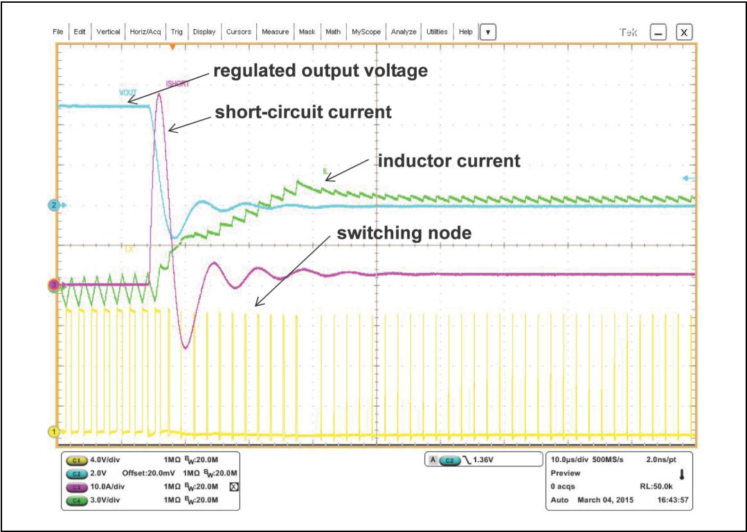
Figure 20. Output voltage oscillations during heavy short-circuit
