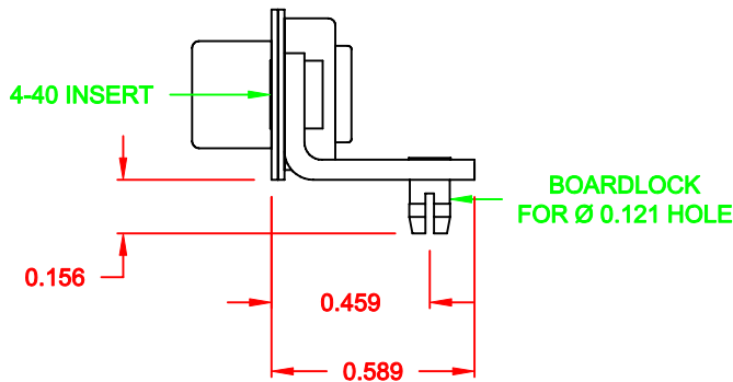
MOUNTING HARDWARE
