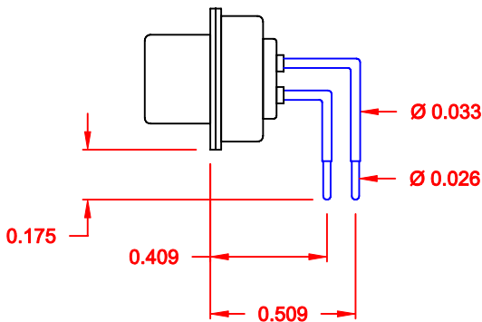
SIGNAL CONTACTS
