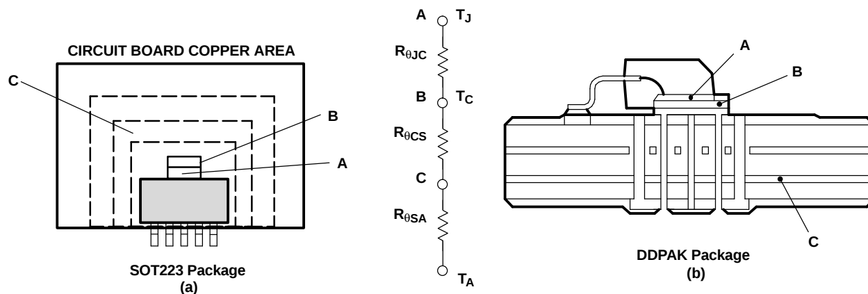
Figure 24. Thermal Resistances
