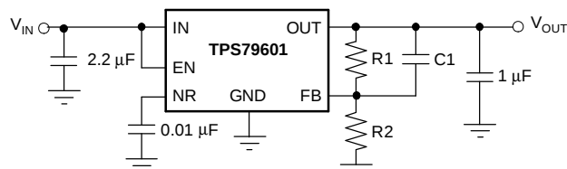
Figure 23. TPS79601 Adjustable LDO Regulator Programming
