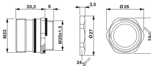
Dimensioned drawing
