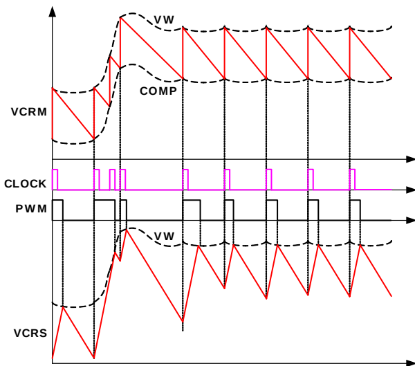
FIGURE 7. R 3 TM MODULATOR OPERATION PRINCIPLES IN LOAD INSERTION RESPONSE
