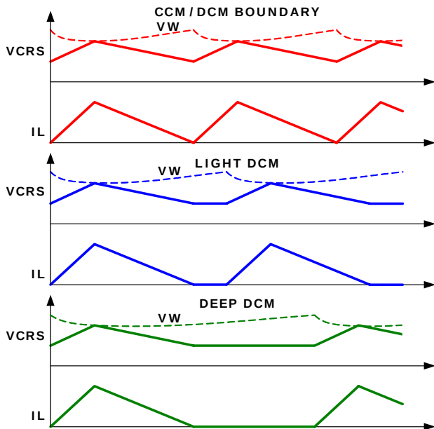
FIGURE 9. PERIOD STRETCHING
