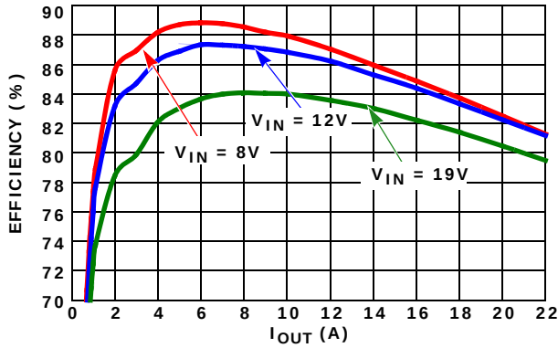
FIGURE 28. ISL62881CCPUEVAL2ZEVALUATION BOARD CCM EFFICIENCY, V_{ID} = 0.9V , V_{IN1} = 8V , V_{IN2} = 12.6V AND V_{IN3} = 19V
