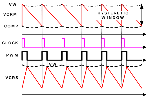
FIGURE 6. R 3 TM MODULATOR OPERATION PRINCIPLES IN STEADY STATE
