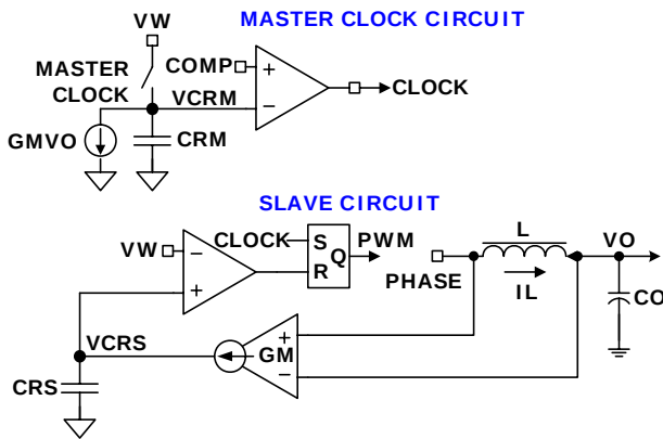
FIGURE 5. R 3 TM MODULATOR CIRCUIT
