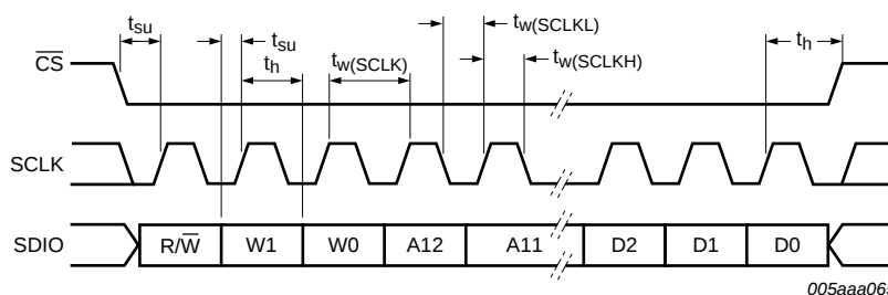
Fig 5. SPI timing
