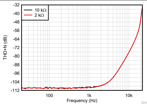
G = 1 , f = 1\text{ kHz} , BW = 80\text{ kHz} , V_{OUT} = 10\text{ V}_{PP} , R_L connected to V_- Figure 5-18. THD+N Ratio vs Frequency, G = 1
