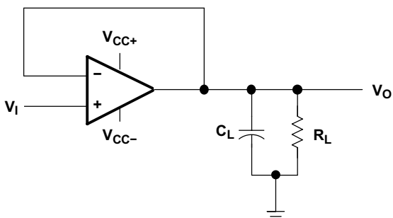
Figure 6-1. Unity-Gain Amplifier
