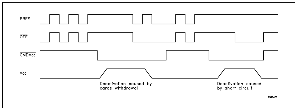
Figure 5 : Behavior of \overline{OFF} , \overline{CMDV_{CC}} , PRES and V CC
