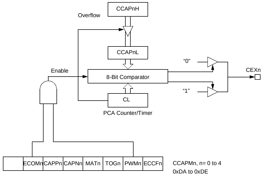
Figure 13. PCA PWM Mode
