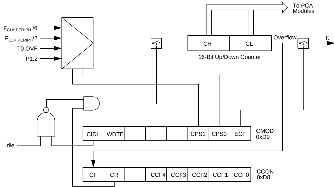
Figure 8. PCA Timer/Counter
