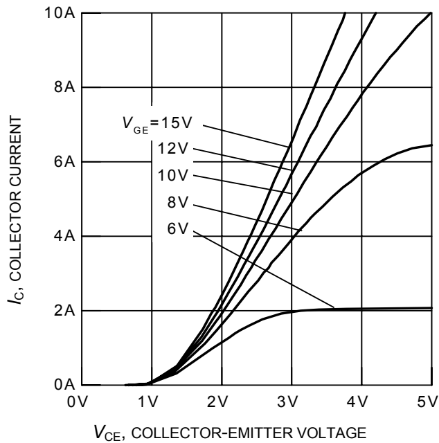
Figure 5. Typical output characteristics ( T_j = 25^\circ C )
