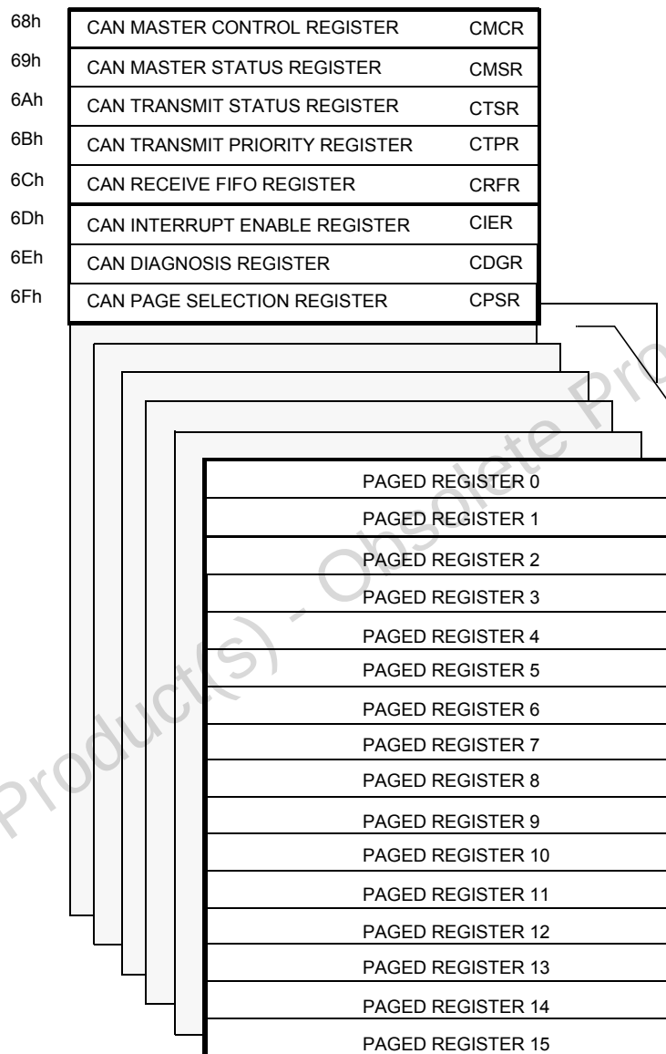
Figure 115. CAN Register Mapping
