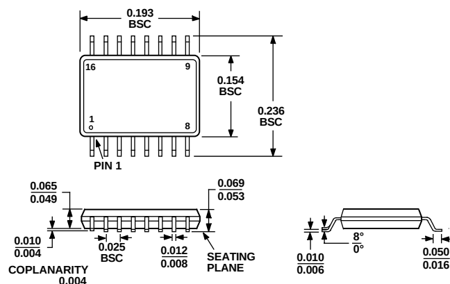
Figure 62. 16-Lead Shrink Small Outline Package [QSOP] (RQ-16)
