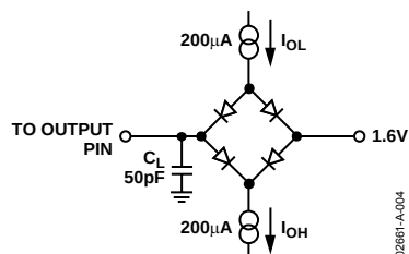
Figure 5. Load Circuit for Access Time and Bus Relinquish Time
