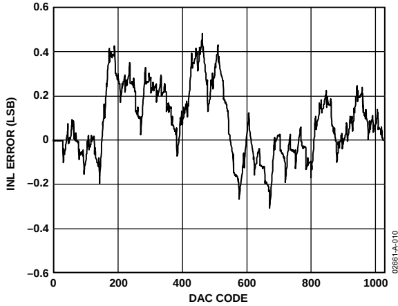
Figure 11. ADT7317 Typical INL Plot
