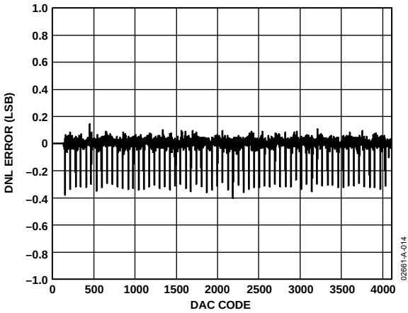
Figure 15. ADT7316 Typical DNL Plot
