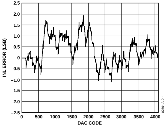
Figure 12. ADT7316 Typical INL Plot
