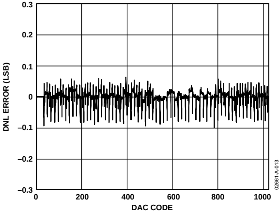
Figure 14. ADT7317 Typical DNL Plot
