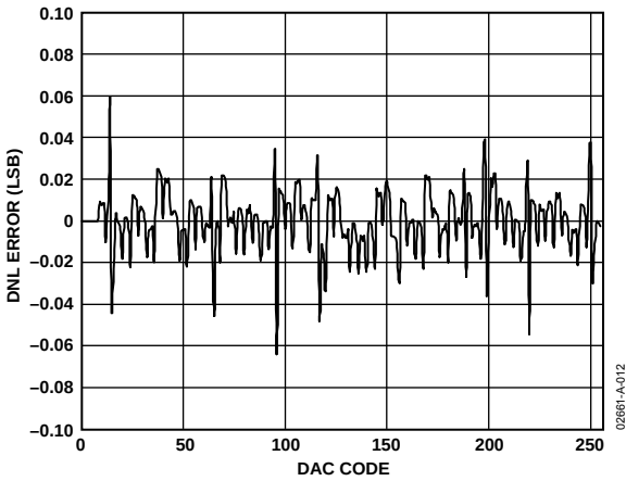
Figure 13. ADT7318 Typical DNL Plot
