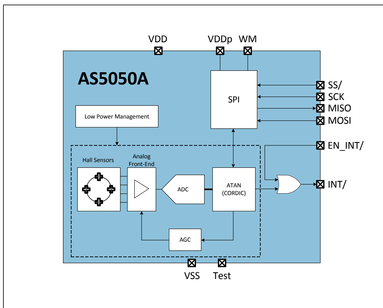
Figure 2: AS5050A Block Diagram
