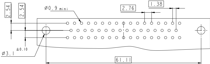
LAYOUT DIMENSIONS
