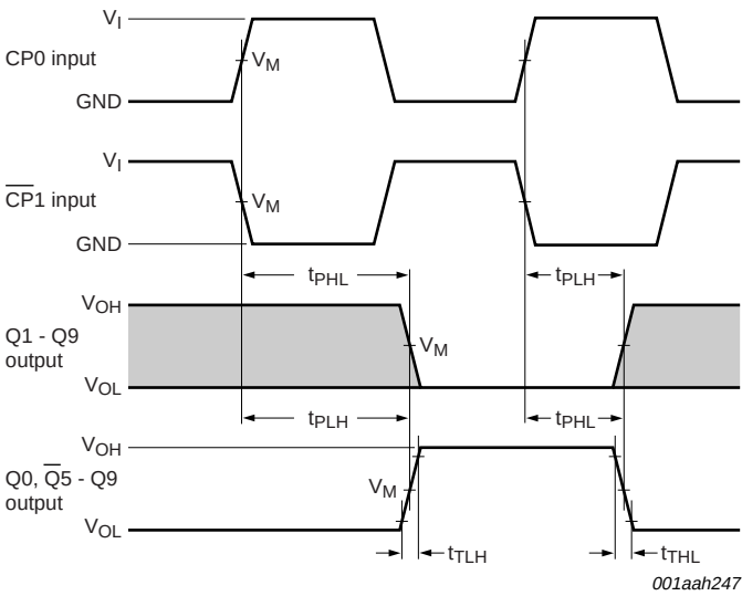
Measurement points are given in Table 8 . V OL and V OH are typical voltage output levels that occur with the output load. Conditions: \overline{CP1} = LOW while CP0 is triggered on a LOW-to-HIGH transition and CP0 = HIGH, while \overline{CP1} is triggered on a HIGH-to-LOW transition.
