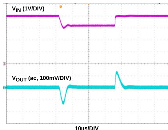
FIGURE 16. 4V TO 3.2V LINE TRANSIENT ( V_{OUT} = 3.3\text{V} , \text{LOAD} = 1\text{A} )
