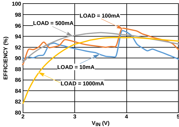
FIGURE 3. EFFICIENCY vs INPUT VOLTAGE
