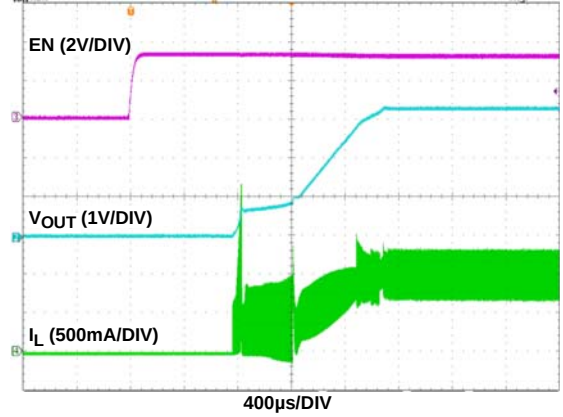
FIGURE 10. SOFT-START ( V_{IN} = 3.6\text{V} , V_{OUT} = 3.3\text{V} , 1A R-LOAD)
