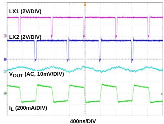
FIGURE 8. STEADY STATE OPERATION IN PWM ( V_{IN} = 3.3\text{V} , V_{OUT} = 3.3\text{V} , NO LOAD)
