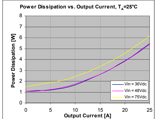
Figure 38. Power Dissipation vs. Load Current at I_O = Full Load, T_A = 25°C (ambient temperature).
