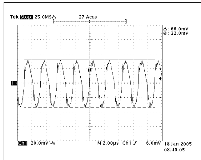
Figure 8. 12V OUT Ripple Waveform at V_{IN} = 48Vdc, I_O = Full Load, T_A = 25°C.
