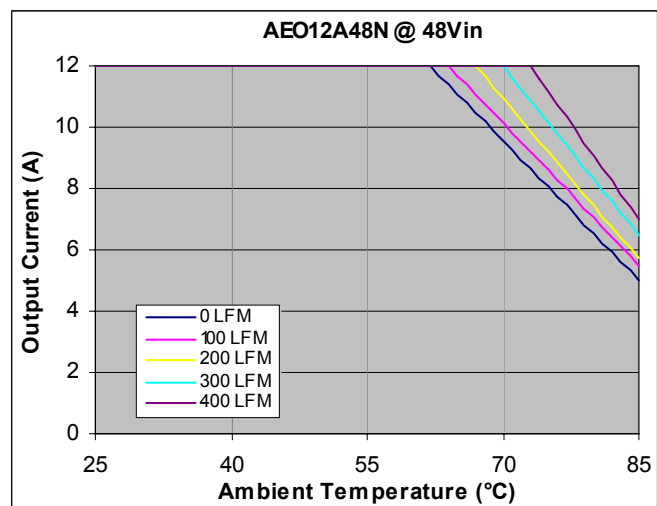
Figure 20. Output Current vs. Temperature for baseplate version at V_{IN} = 48V_{dc} , T_A = 25^\circ\text{C} .
