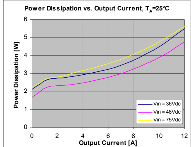
Figure 14. Power Dissipation vs. Load Current at I_O = Full Load, T_A = 25°C (ambient temperature).
