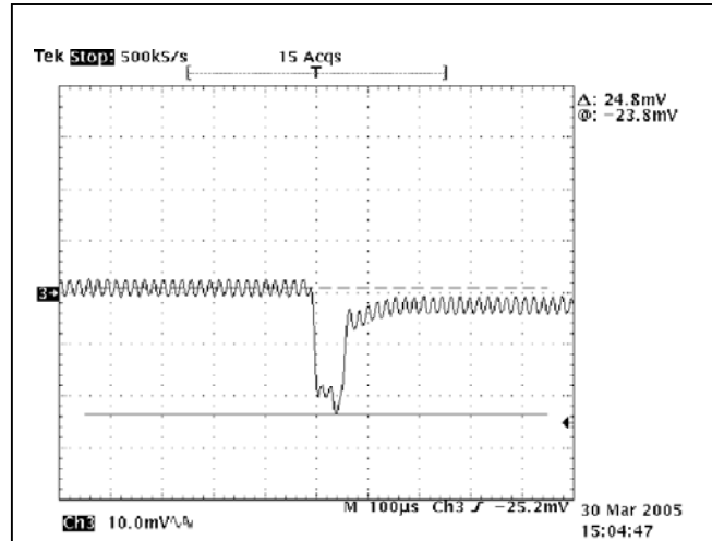
Figure 42. Transient Response at T_A = 25^\circ\text{C} , 1.8V_{OUT} Deviation (Lo-Hi).
