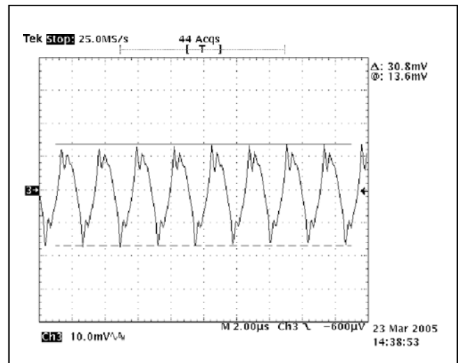
Figure 48. 1.5V OUT Ripple Waveform at V_{IN} = 48Vdc, I_O = Full Load, T_A = 25°C.
