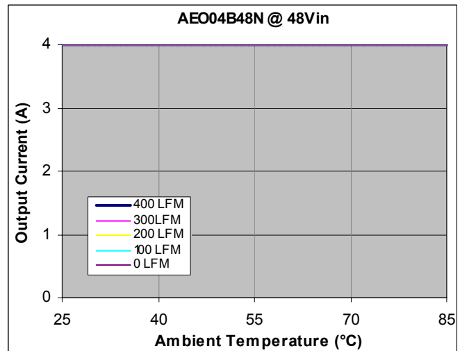
Figure 12. Output Current vs. Temperature for baseplate version at V_{IN} = 48\text{Vdc} , T_A = 25^\circ\text{C} .
