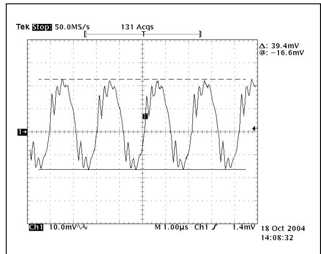
Figure 16. 5V OUT Ripple Waveform at V_{IN} = 48Vdc, I_O = Full Load, T_A = 25°C.
