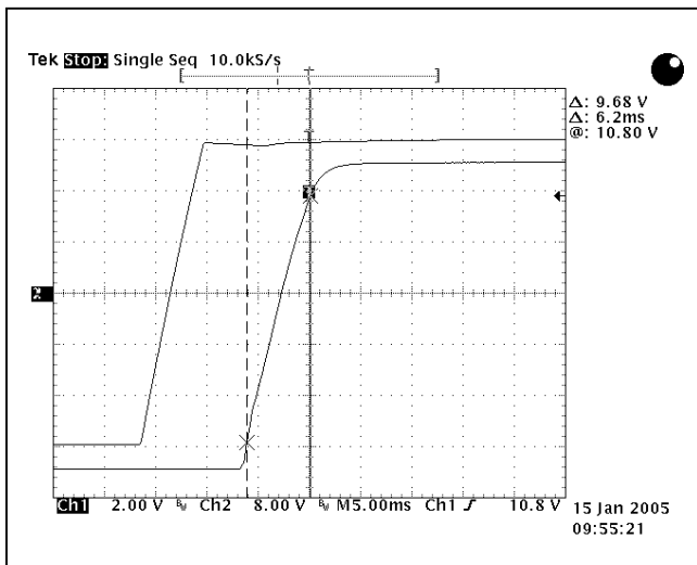
Figure 7. 12V OUT Startup Characteristic at V_{IN} = 48Vdc, I_O = Full Load, T_A = 25°C.
