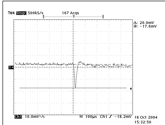
Figure 18. Transient Response at T_A = 25^\circ\text{C} , 5V_{OUT} Deviation (Lo-Hi).
