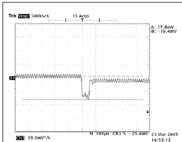
Figure 50. Transient Response at T_A = 25^\circ\text{C} , 1.5V_{OUT} Deviation (Lo-Hi).
