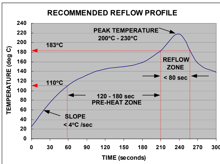
Figure 64. Recommended reflow profile for SMT modules.
