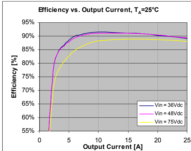
Figure 37. Efficiency vs. Load Current at I_O = Full Load, T_A = 25°C (ambient temperature).
