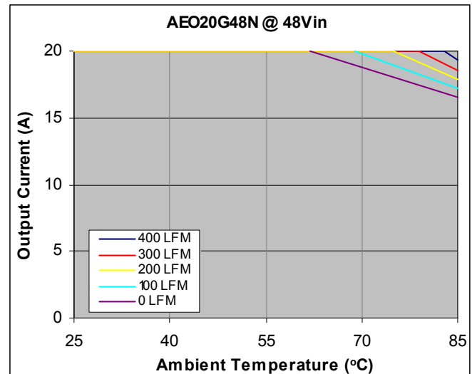
Figure 36. Output Current vs. Temperature for baseplate version at V_{IN} = 48\text{Vdc} , T_A = 25^\circ\text{C} .
