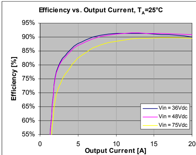
Figure 29. Efficiency vs. Load Current at I_O = Full Load, T_A = 25^\circ\text{C} (ambient temperature).
