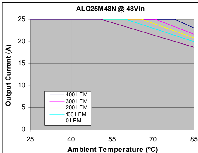
Figure 51. Output Current vs. Temperature for open frame version at V_{IN} = 48\text{Vdc} , T_A = 25^\circ\text{C} .
