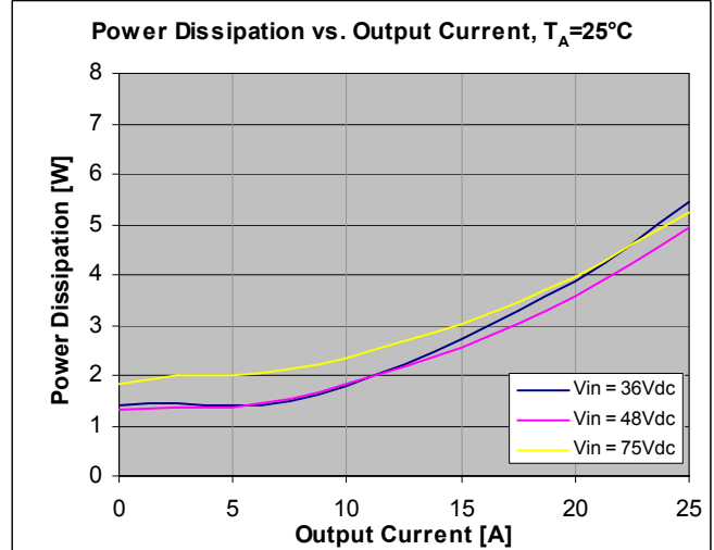
Figure 46. Power Dissipation vs. Load Current at I_O = Full Load, T_A = 25°C (ambient temperature).
