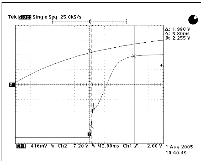
Figure 31. 2.5V OUT Startup Characteristic at V_{IN} = 48\text{Vdc} , I_O = Full Load, T_A = 25^\circ\text{C} .
