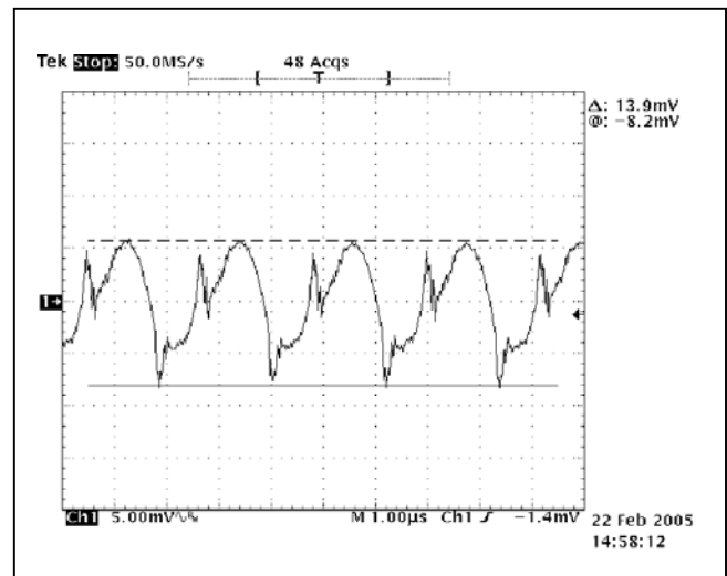
Figure 56. 1.2 V OUT Ripple Waveform at V_{IN} = 48Vdc, I_O = Full Load, T_A = 25°C.
