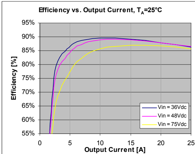
Figure 53. Efficiency vs. Load Current at I_O = Full Load, T_A = 25°C (ambient temperature).
