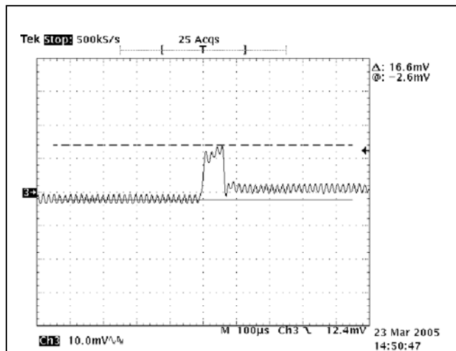
Figure 49. Transient Response at T_A = 25^\circ\text{C} , 1.5V_{OUT} Deviation (Hi-Lo).
