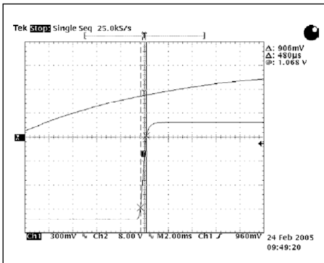
Figure 55. 1.2V OUT Startup Characteristic at V_{IN} = 48Vdc, I_O = Full Load, T_A = 25°C.
