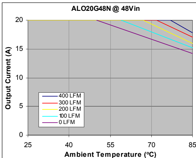
Figure 35. Output Current vs. Temperature for open frame version at V_{IN} = 48\text{Vdc} , T_A = 25^\circ\text{C} .
