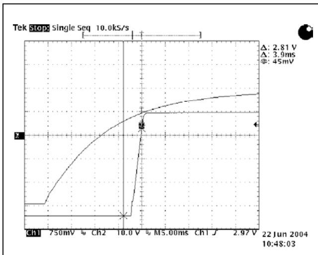
Figure 23. 3.3V OUT Startup Characteristic at V_{IN} = 48Vdc, I_O = Full Load, T_A = 25°C.
