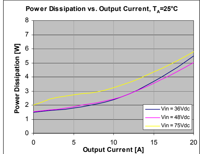
Figure 30. Power Dissipation vs. Load Current at I_O = Full Load, T_A = 25^\circ\text{C} (ambient temperature).
