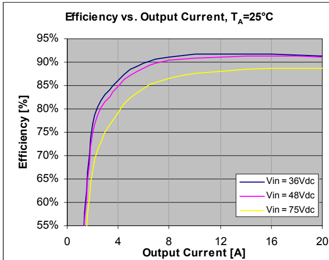
Figure 21. Efficiency vs. Load Current at I_O = Full Load, T_A = 25°C (ambient temperature).
