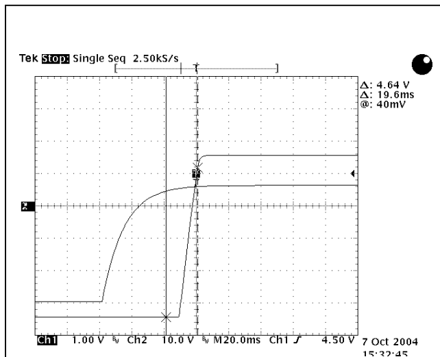
Figure 15. 5V OUT Startup Characteristic at V_{IN} = 48Vdc, I_O = Full Load, T_A = 25°C.
