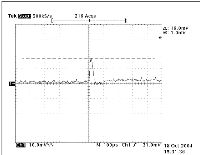
Figure 17. Transient Response at T_A = 25^\circ\text{C} , 5V_{OUT} Deviation (Hi-Lo).
