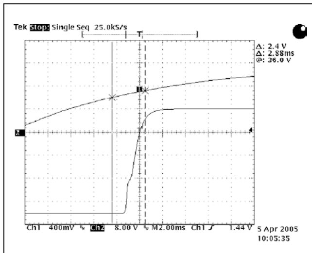
Figure 39. 1.8V OUT Startup Characteristic at V_{IN} = 48Vdc, I_O = Full Load, T_A = 25°C.
