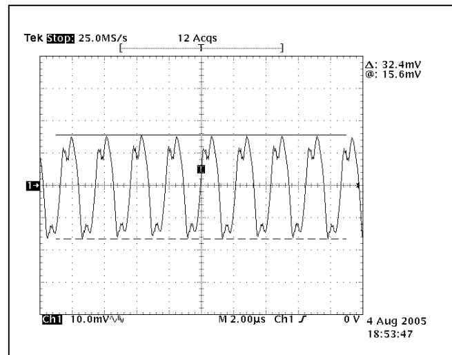
Figure 32. 2.5V OUT Ripple Waveform at V_{IN} = 48\text{Vdc} , I_O = Full Load, T_A = 25^\circ\text{C} .
