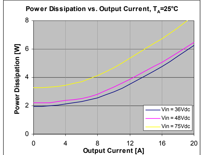
Figure 22. Power Dissipation vs. Load Current at I_O = Full Load, T_A = 25°C (ambient temperature).
