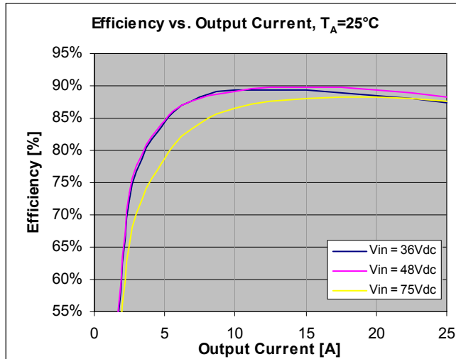
Figure 45. Efficiency vs. Load Current at I_O = Full Load, T_A = 25°C (ambient temperature).
