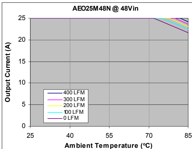
Figure 52. Output Current vs. Temperature for baseplate version at V_{IN} = 48\text{Vdc} , T_A = 25^\circ\text{C} .
