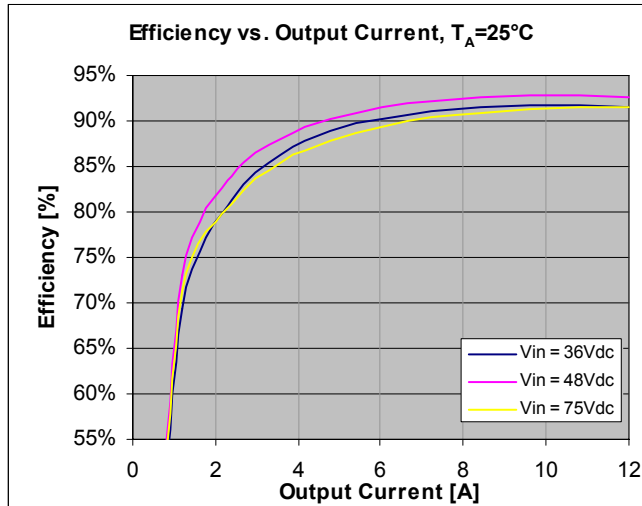
Figure 13. Efficiency vs. Load Current at I_O = Full Load, T_A = 25°C (ambient temperature).
