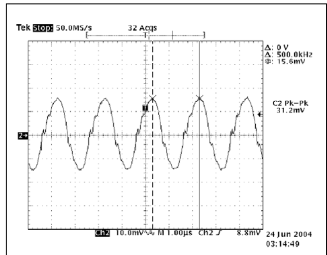
Figure 24. 3.3V OUT Ripple Waveform at V_{IN} = 48Vdc, I_O = Full Load, T_A = 25°C.
