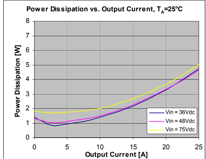
Figure 54. Power Dissipation vs. Load Current at I_O = Full Load, T_A = 25°C (ambient temperature).
