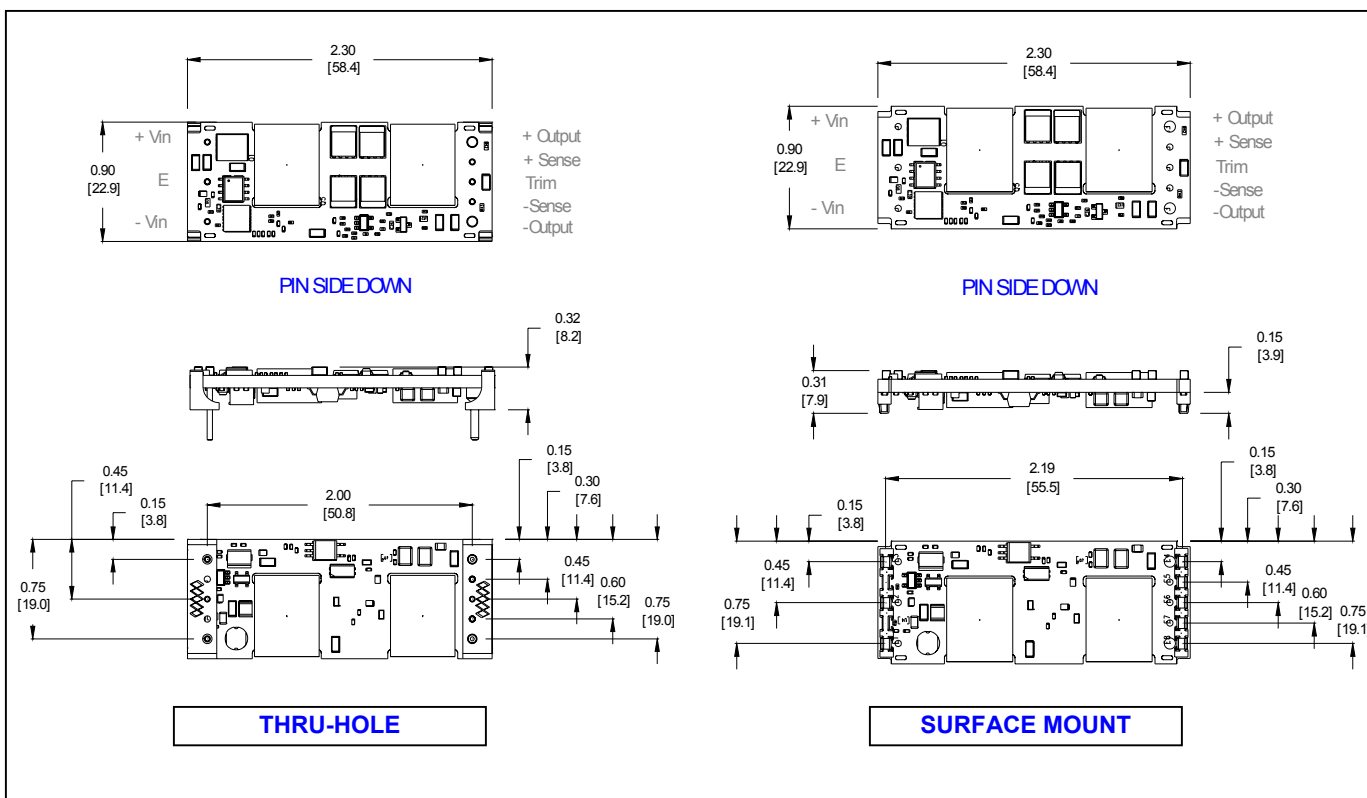
Figure 62A. ALO (Openframe) Mechanical outline.
