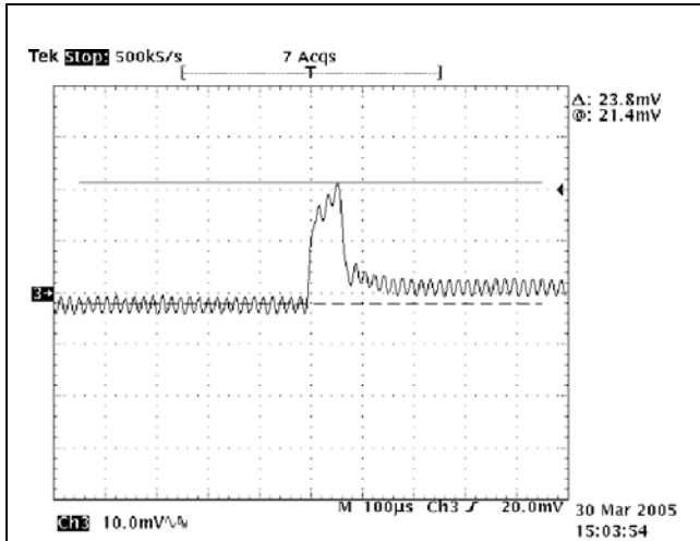
Figure 41. Transient Response at T_A = 25^\circ\text{C} , 1.8V_{OUT} Deviation (Hi-Lo).
