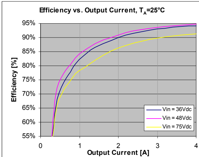
Figure 5. Efficiency vs. Load Current at I_O = Full Load, T_A = 25°C (ambient temperature).
