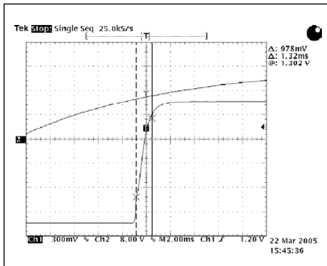
Figure 47. 1.5V OUT Startup Characteristic at V_{IN} = 48Vdc, I_O = Full Load, T_A = 25°C.
