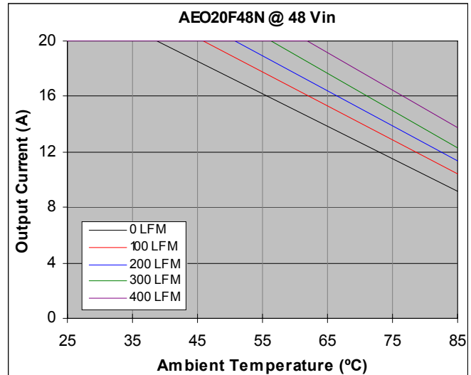
Figure 28. Output Current vs. Temperature for baseplate version at V_{IN} = 48\text{Vdc} , T_A = 25^\circ\text{C} .
