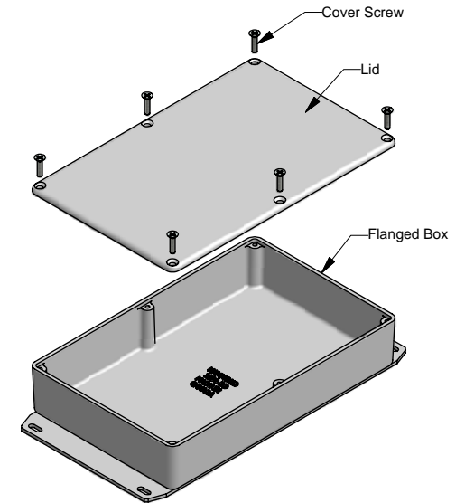
Series 1590DD (Flanged Box)
