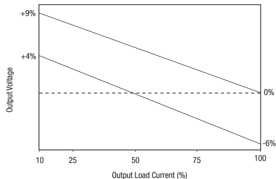
Short circuit
