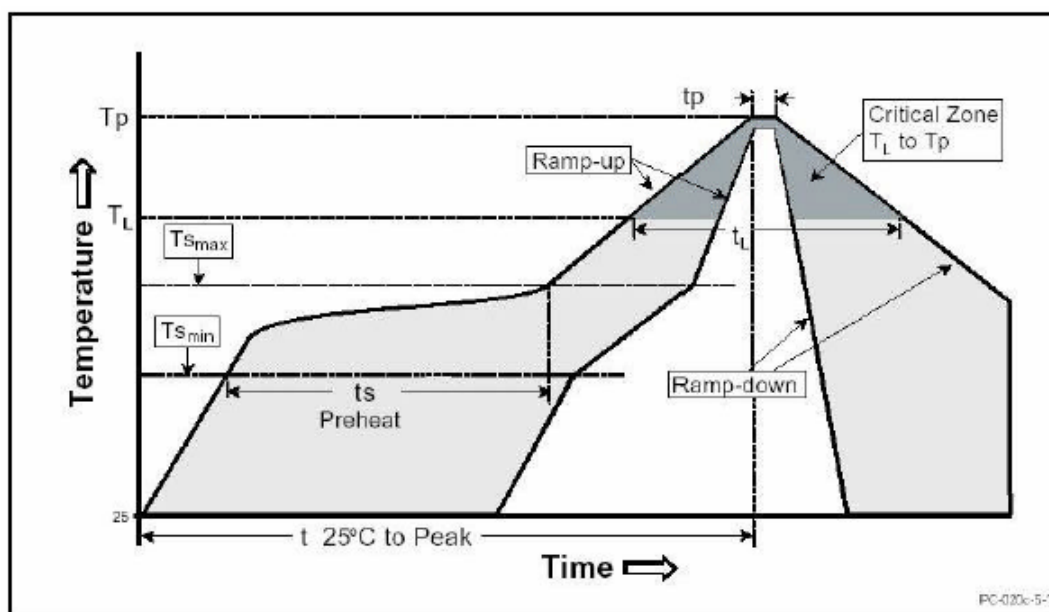
Figure 7. Solder Reflow Profile
