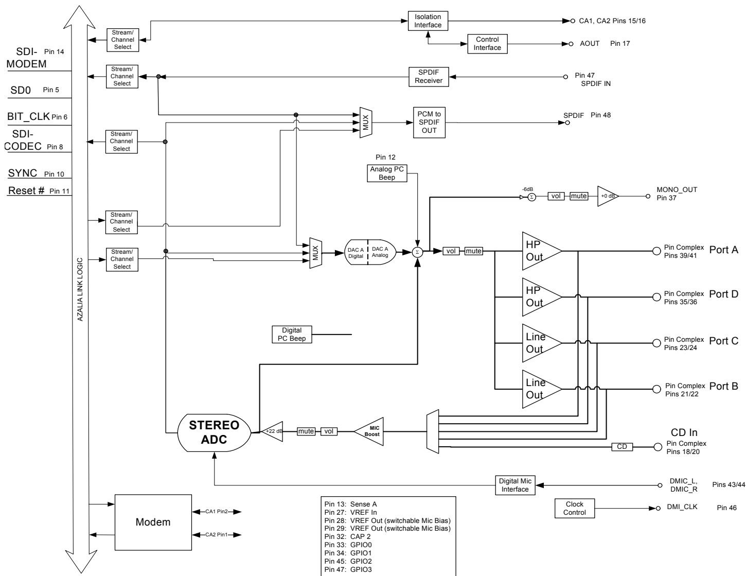
Figure 2. STAC9250 Functional Block Diagram
