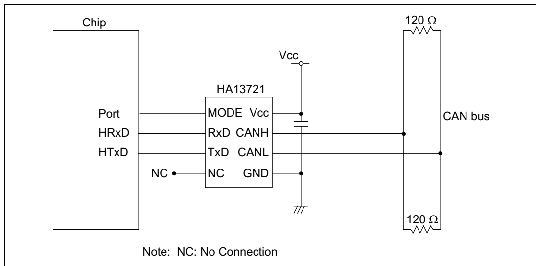
Figure 16-14 High-Speed Interface Using HA13721
