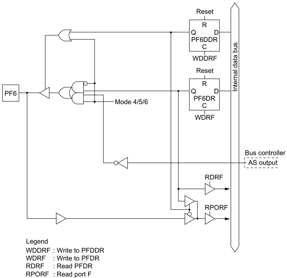
Figure C-10 (e) Port F Block Diagram (Pin PF6)
