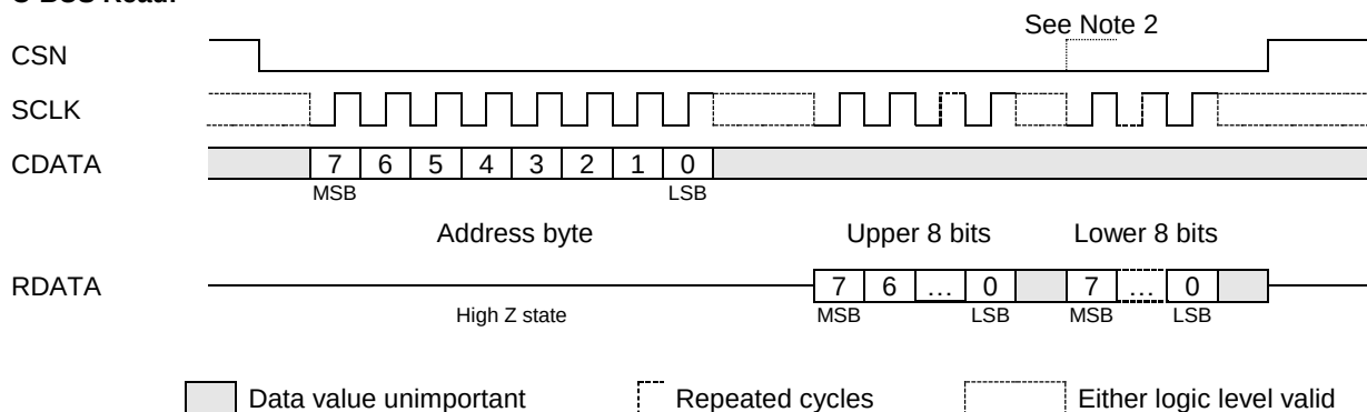
Figure 6 C-BUS Transactions
