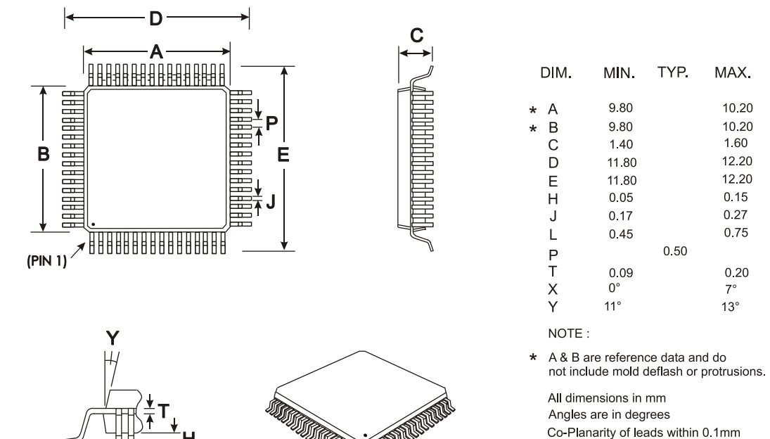
Figure 22 Mechanical Outline for 64-pin LQFP (leaded) Package (L9)
