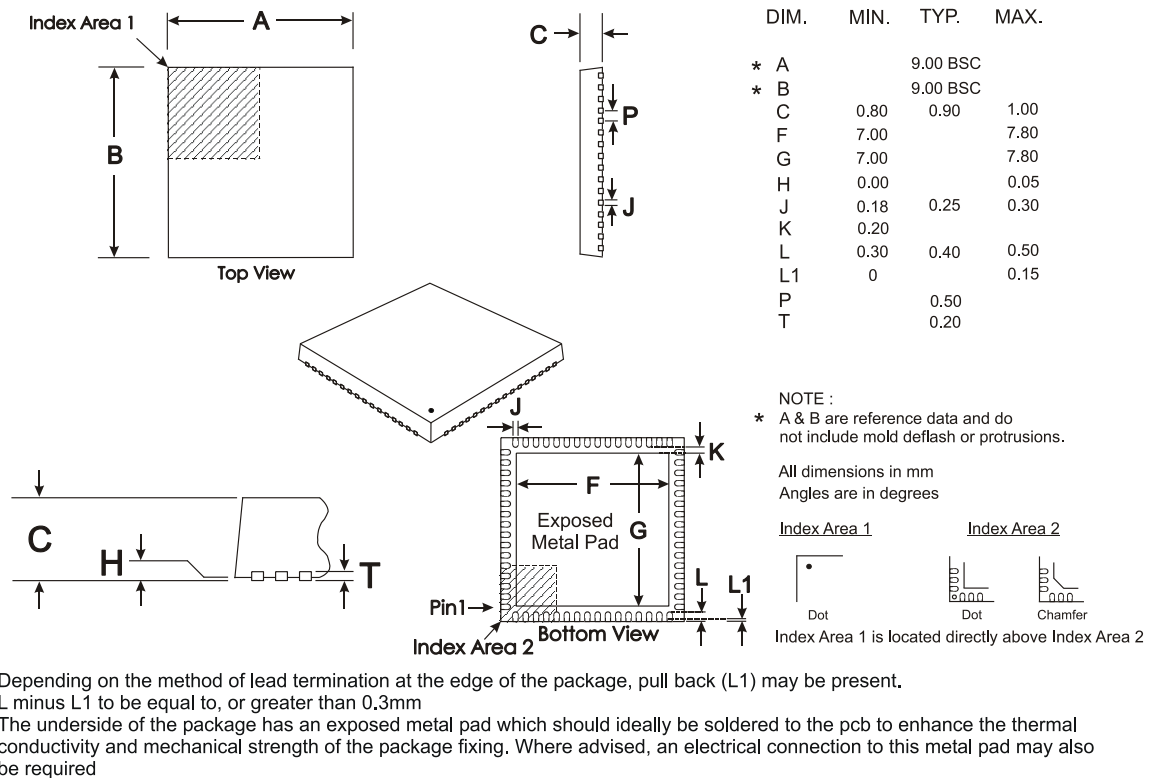
Figure 21 Mechanical Outline for 64-pad VQFN Package (Q1)
