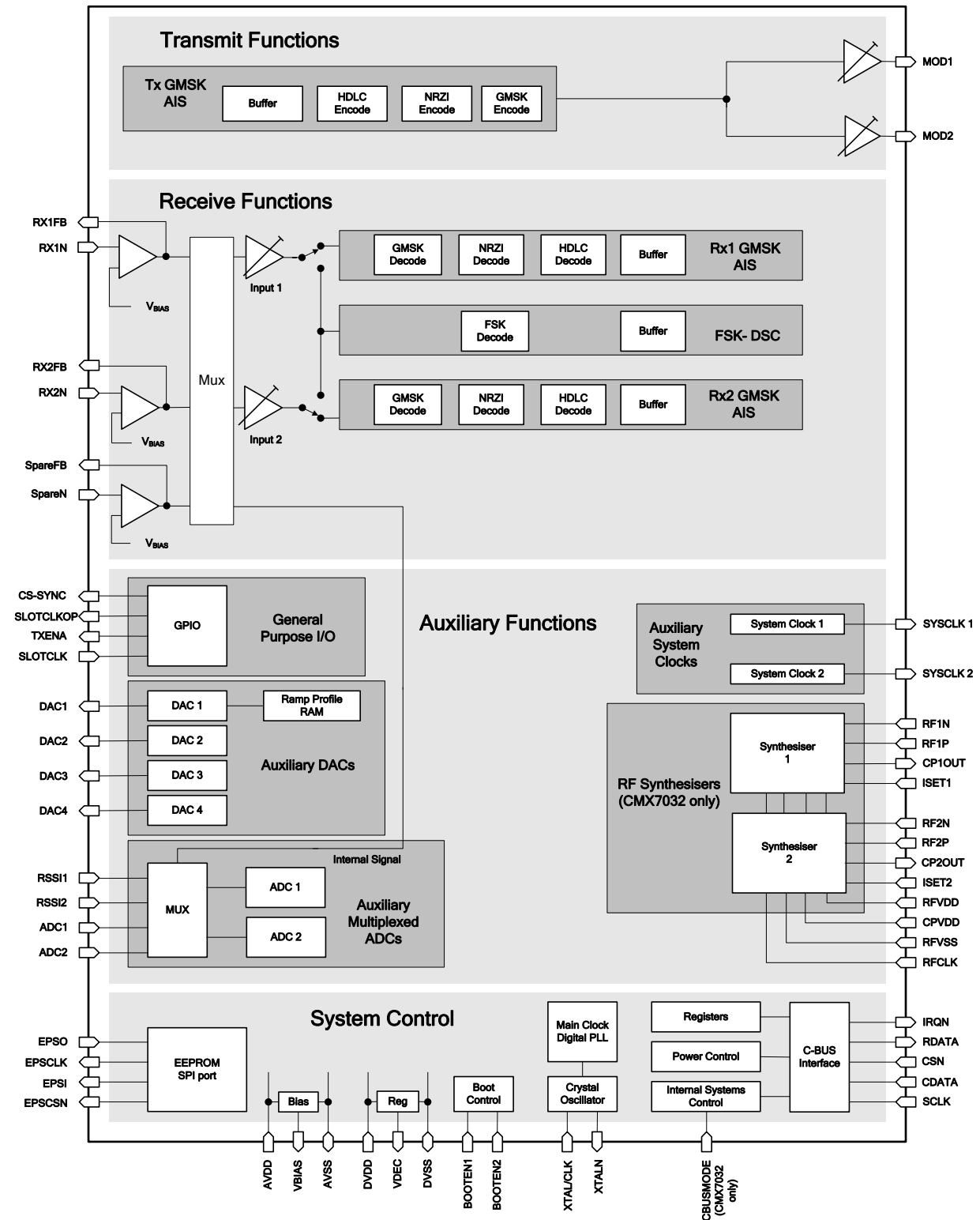
Figure 1 CMX7032/CMX7042 Block Diagram
