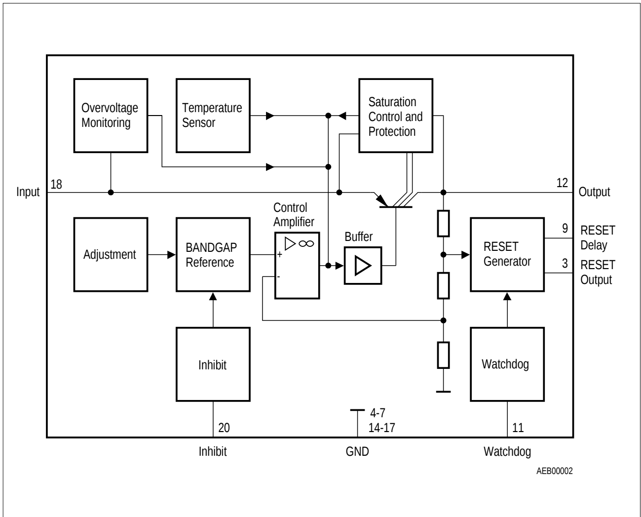
Block Diagram
