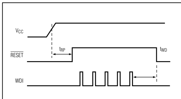
Figure 4. Watchdog Timing
