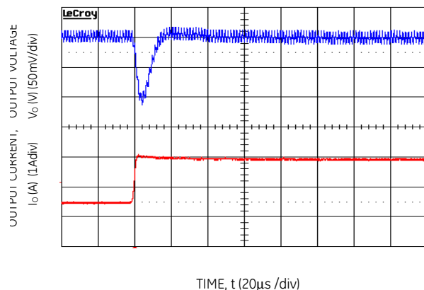
Figure 34. Transient Response to Dynamic Load Change from 50% to 100% at 12V in , C_{out}=1\mu\text{F} , C_{Tune}=820\text{pF} & RTune-261
