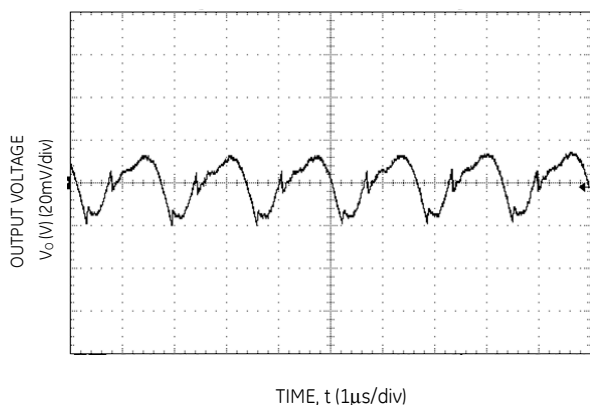
Figure 27. Typical output ripple and noise ( C_o=10\mu\text{F} ceramic, V_{IN} = 12\text{V} , I_o = I_{o,max} ).
