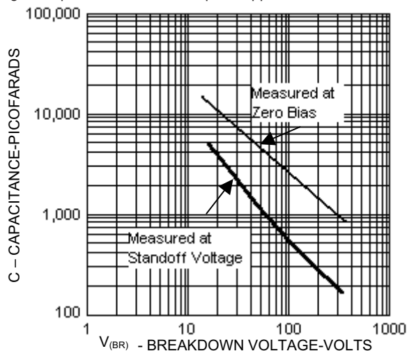
Typical Capacitance vs. Breakdown Voltage
