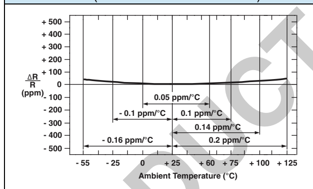
FIGURE 3 - TYPICAL TCR CURVE Z-FOIL (for more details see table 1)
