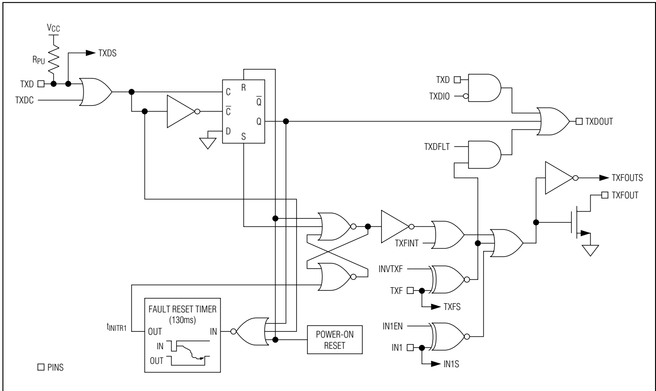
Figure 10. Logic Diagram 1
