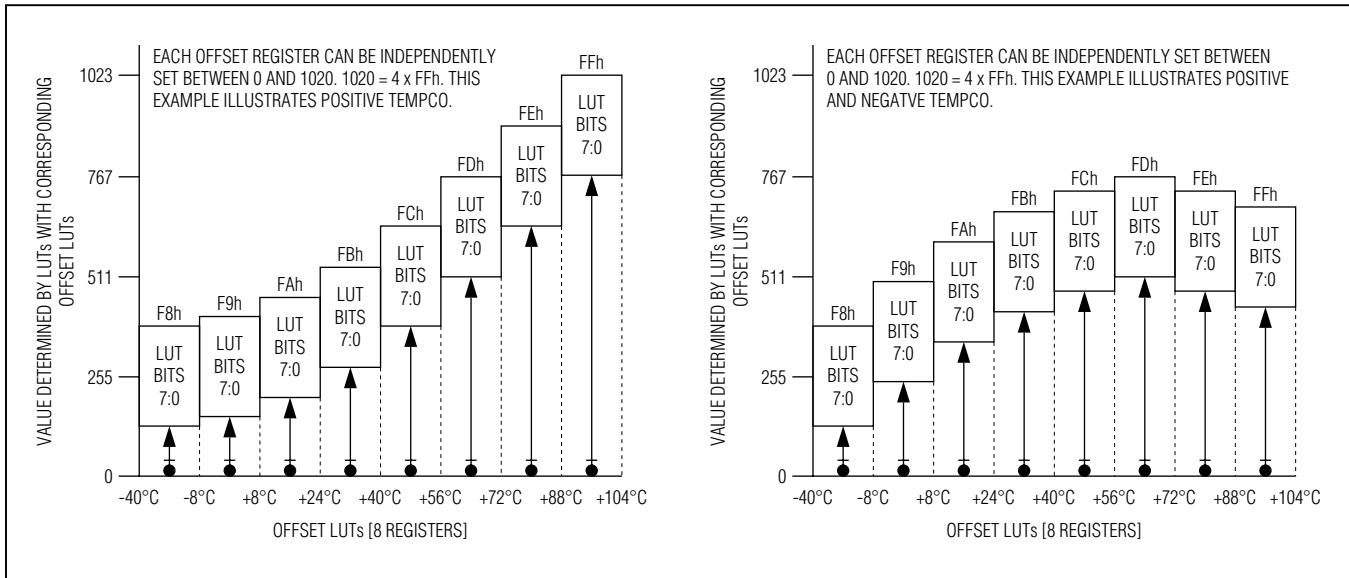
Figure 15. Offset LUT
