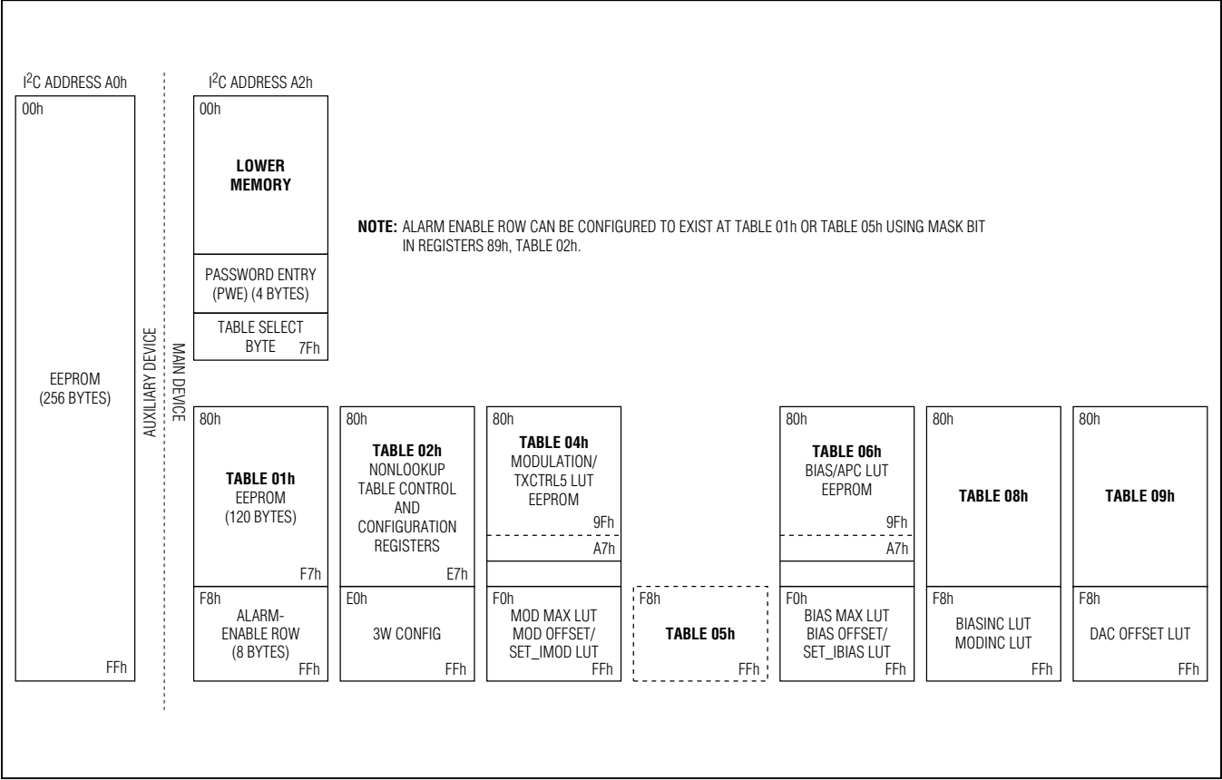
Figure 20. Memory Organization
