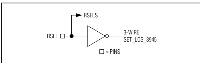
Figure 11. Logic Diagram 2
