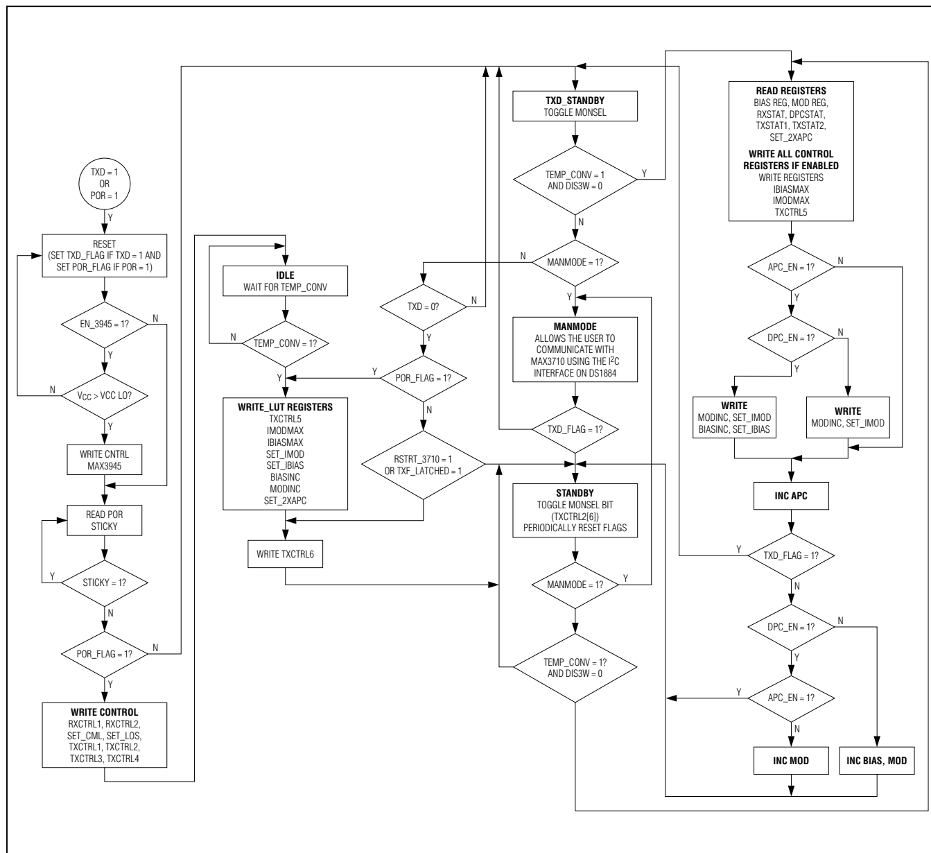
Figure 14. 3-Wire Flowchart
