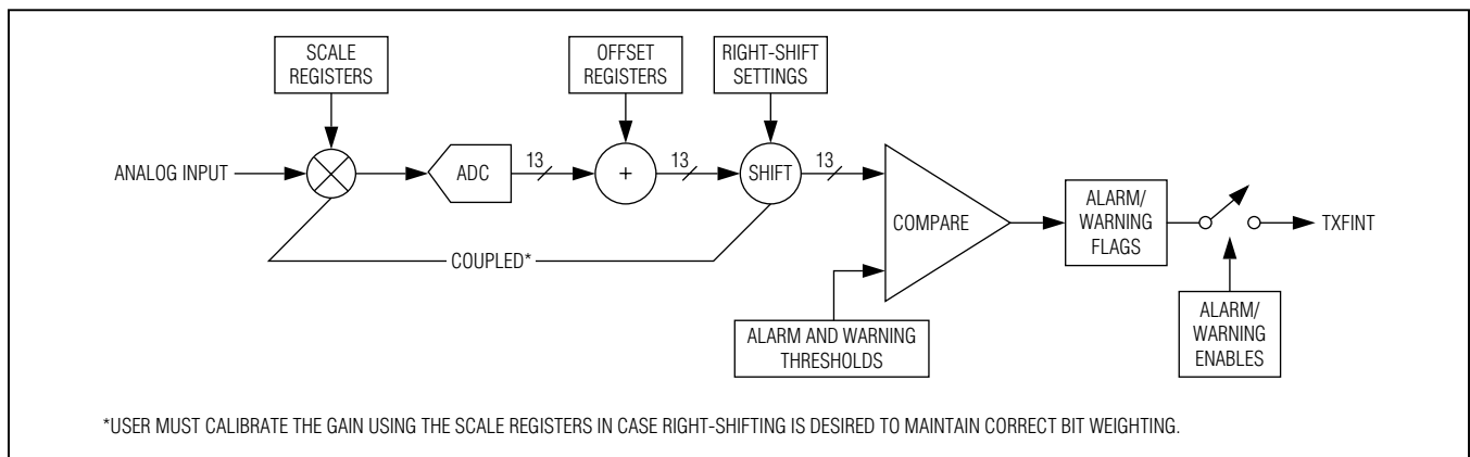
Figure 1. ADC Channel
