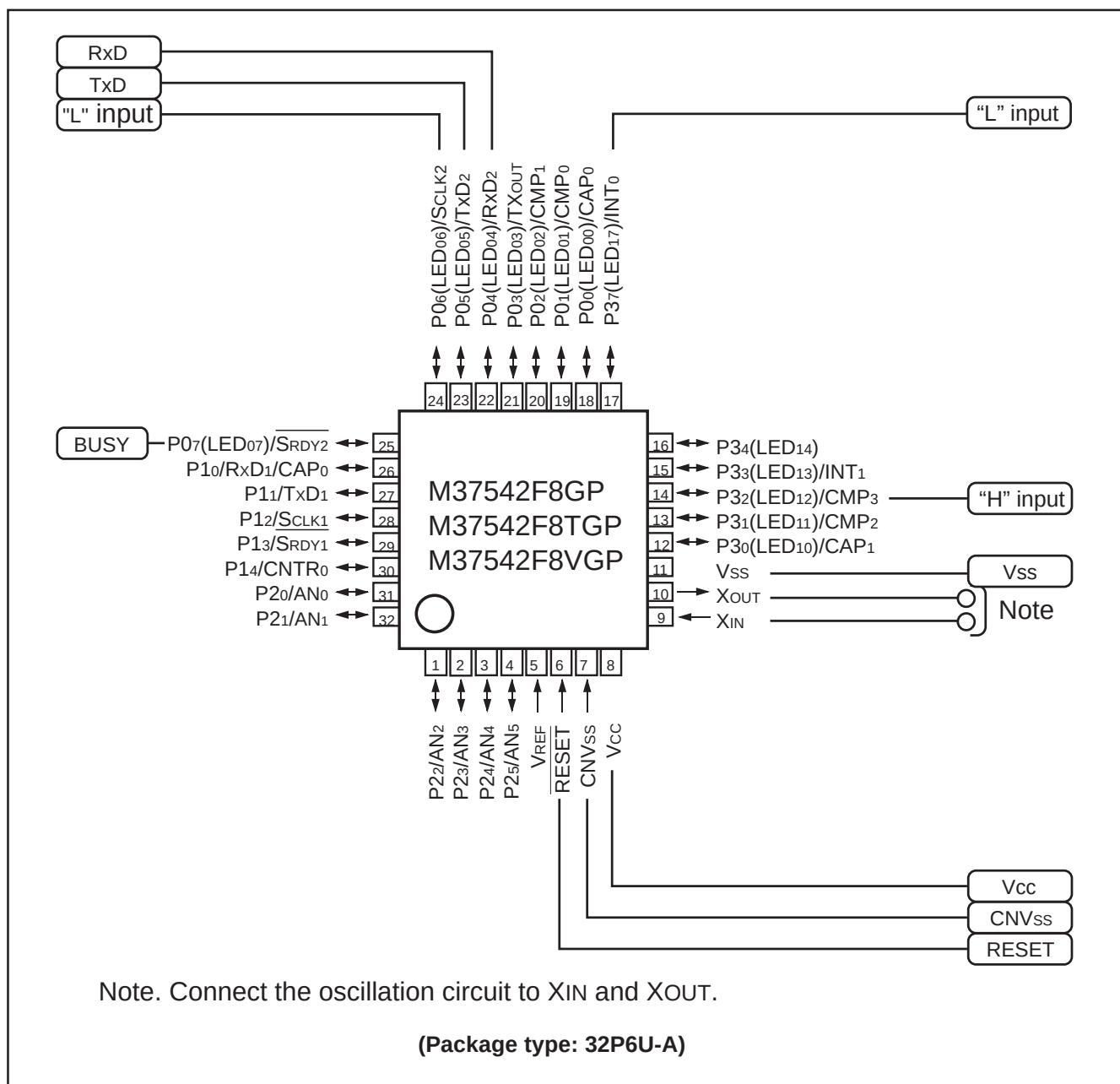
Fig. 109 Pin connection diagram in standard serial I/O mode 2 (32P6U-A package)
