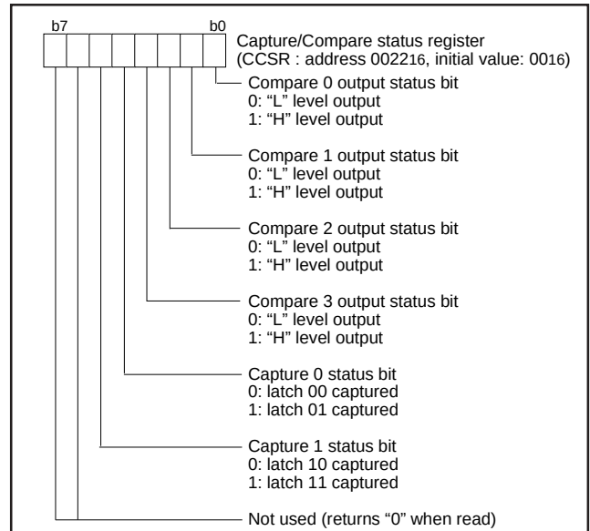
Fig. 37 Structure of capture/compare status register
