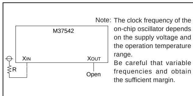
Fig. 73 Processing of X_{IN} and X_{OUT} pins at on-chip oscillator operation
