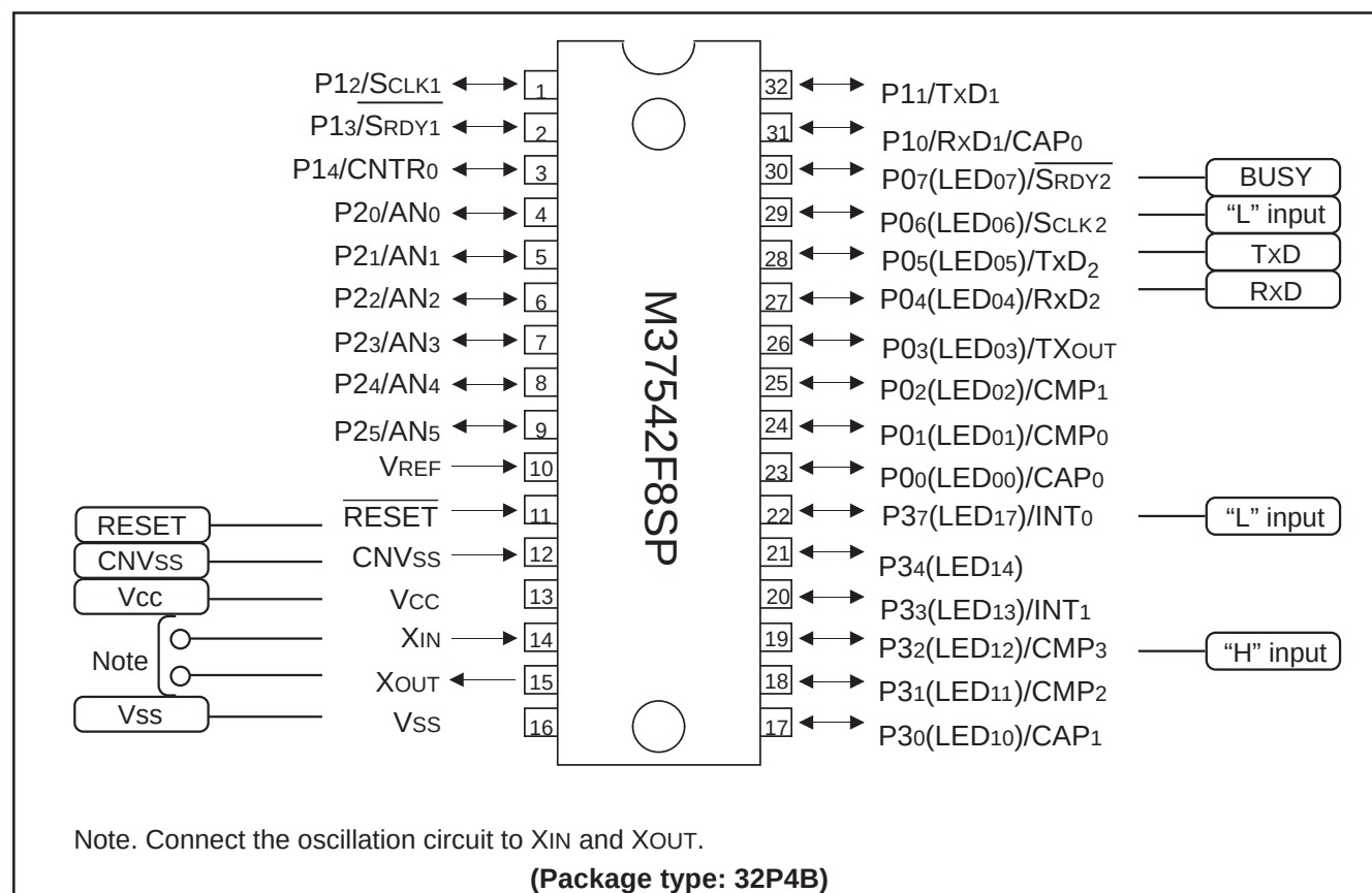
Fig. 111 Pin connection diagram in standard serial I/O mode 2 (32P4B package)
