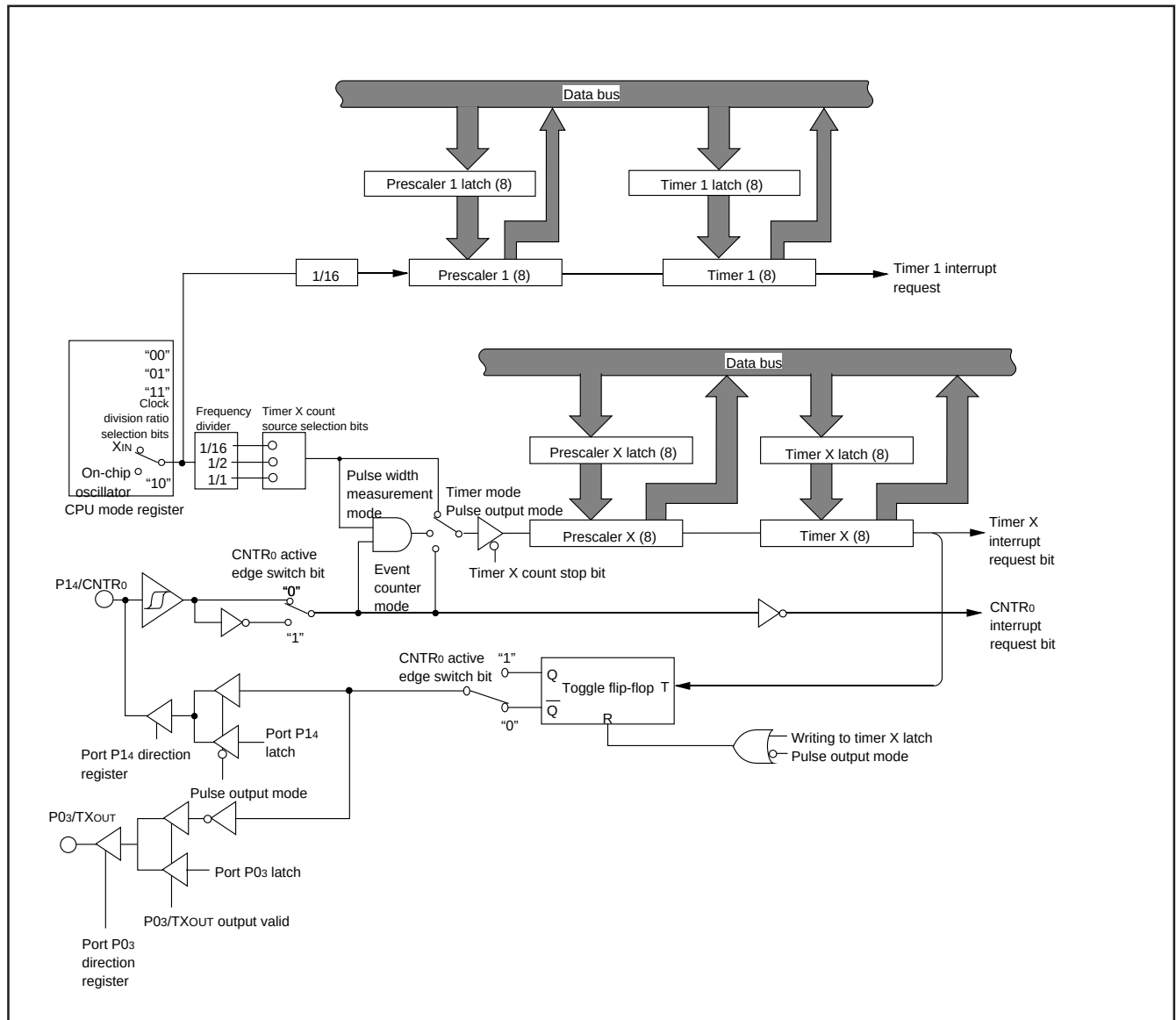
Fig. 28 Block diagram of timer 1 and timer X
