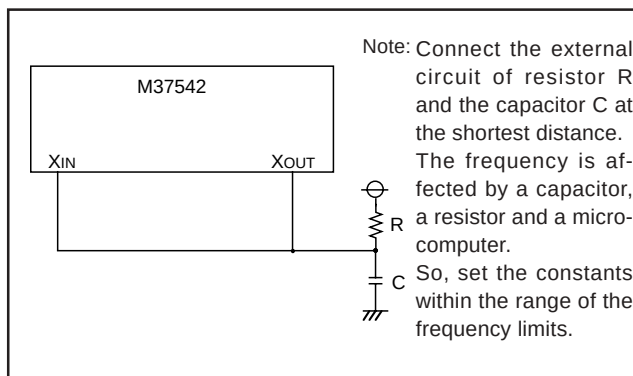
Fig. 75 External circuit of RC oscillation
