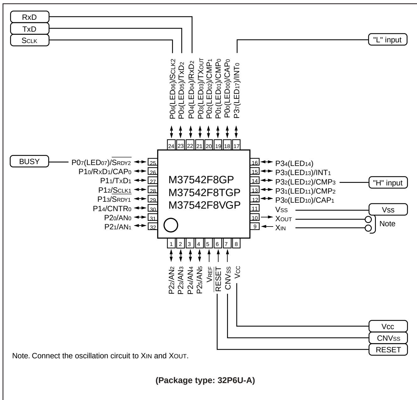
Fig. 104 Pin connection diagram in standard serial I/O mode 1 (32P6U-A package)
