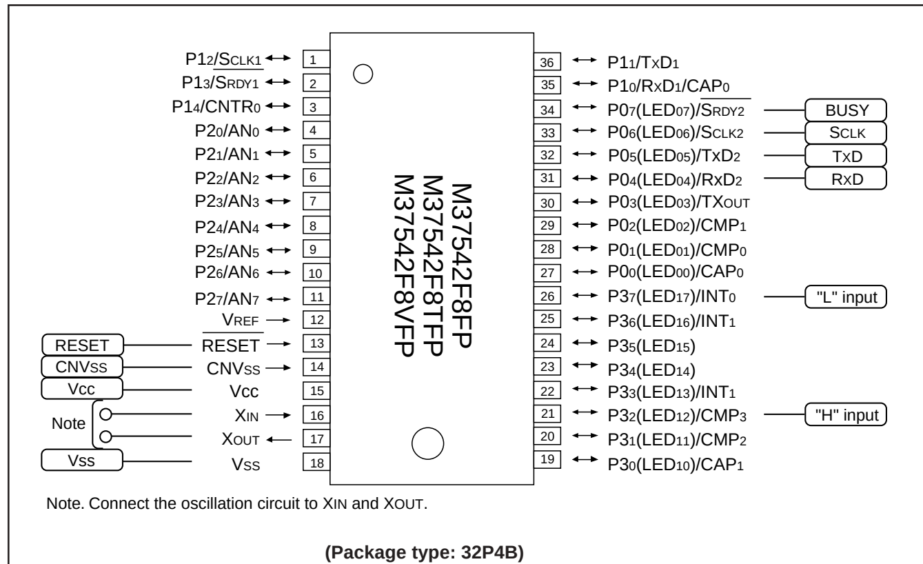
Fig. 106 Pin connection diagram in standard serial I/O mode 1 (32P4B package)
