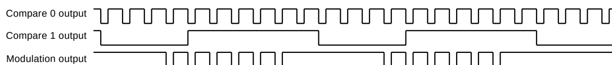
Fig. 45 Output compare mode (compare 0, 1 modulation mode: effect of output level latch)
