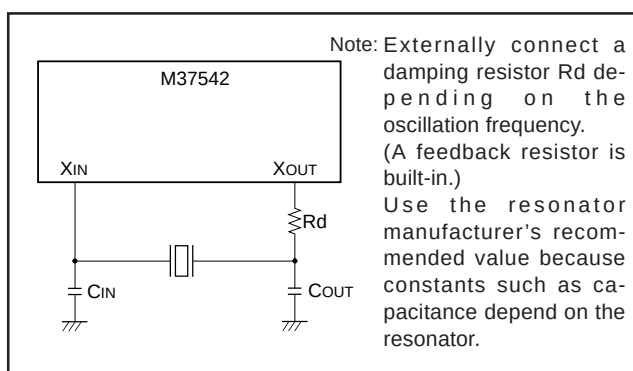
Fig. 74 External circuit of ceramic resonator
