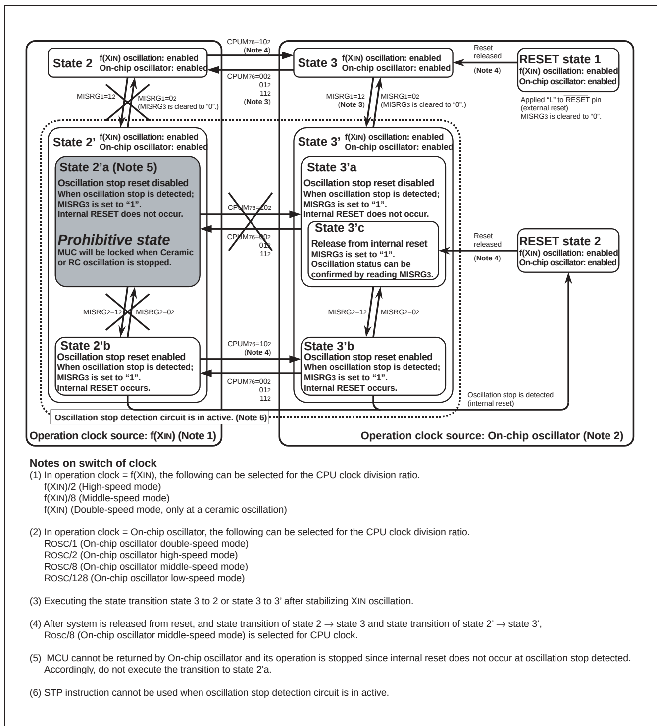
Fig. 83 State transition 2
