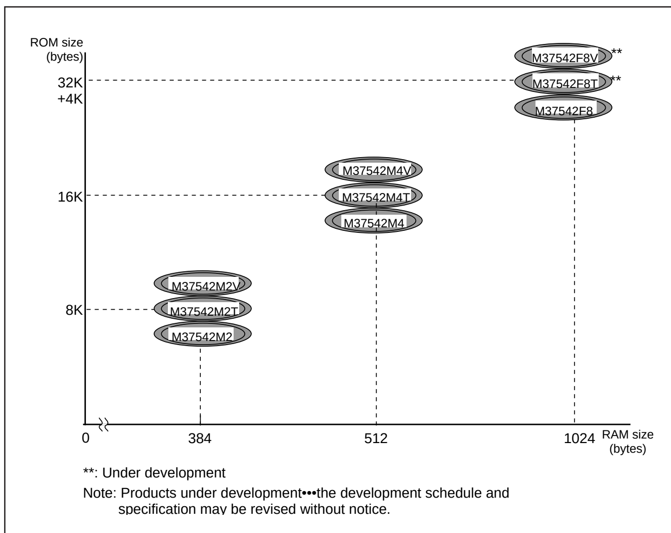
Fig. 10 Memory expansion plan
