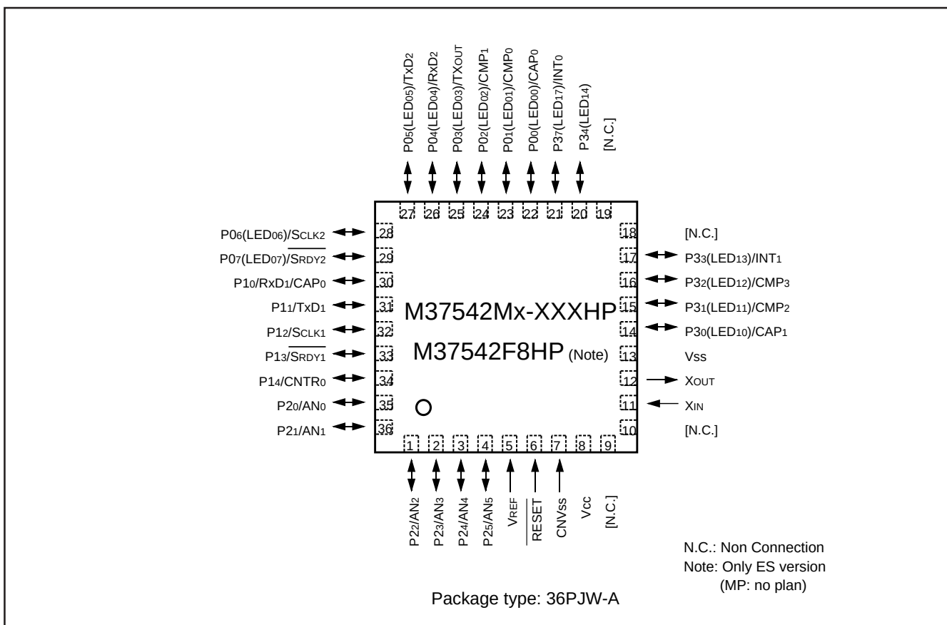
Fig. 4 Pin configuration ((Package type: 36PJW-A)
