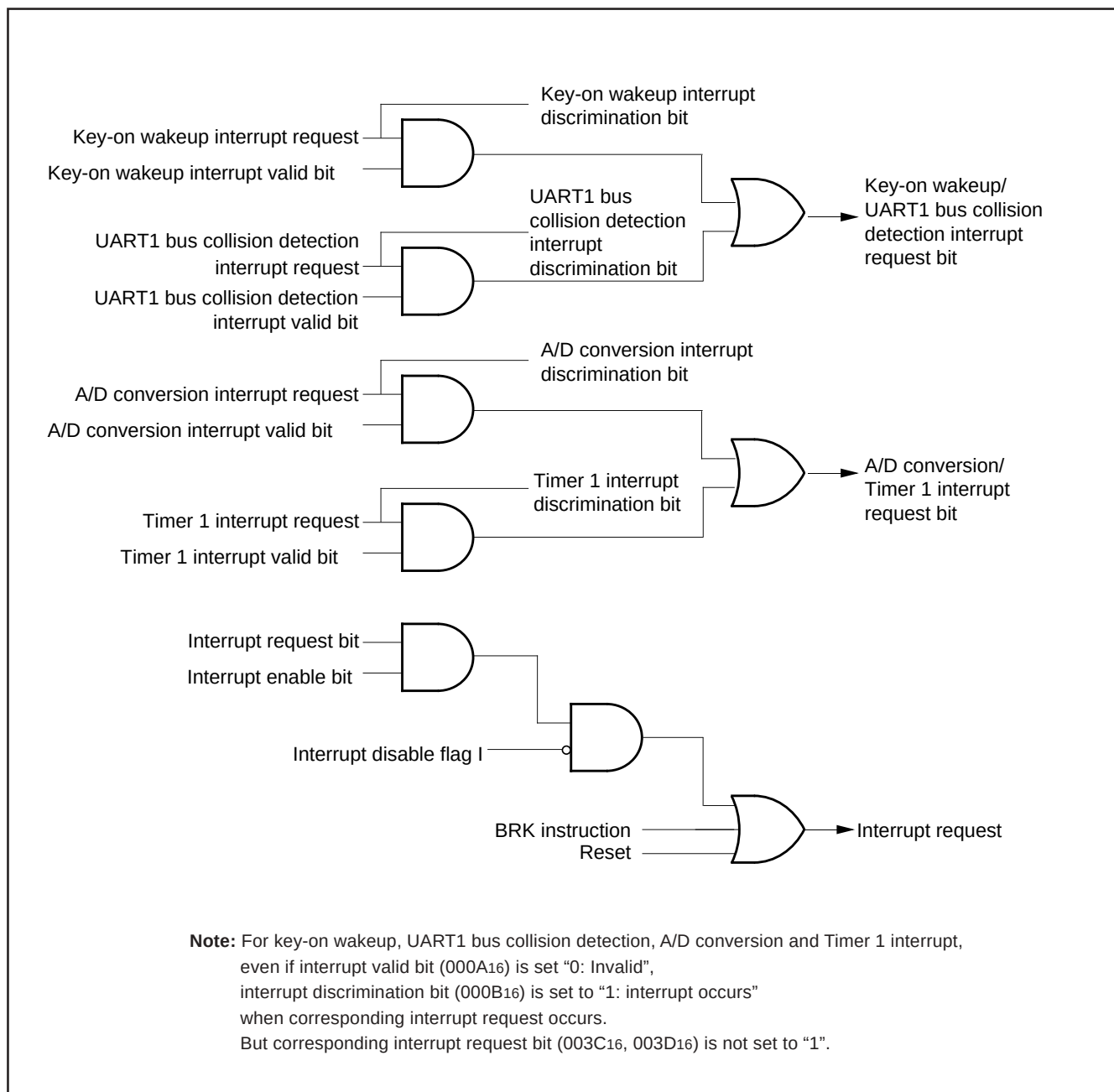
Fig. 23 Interrupt control
