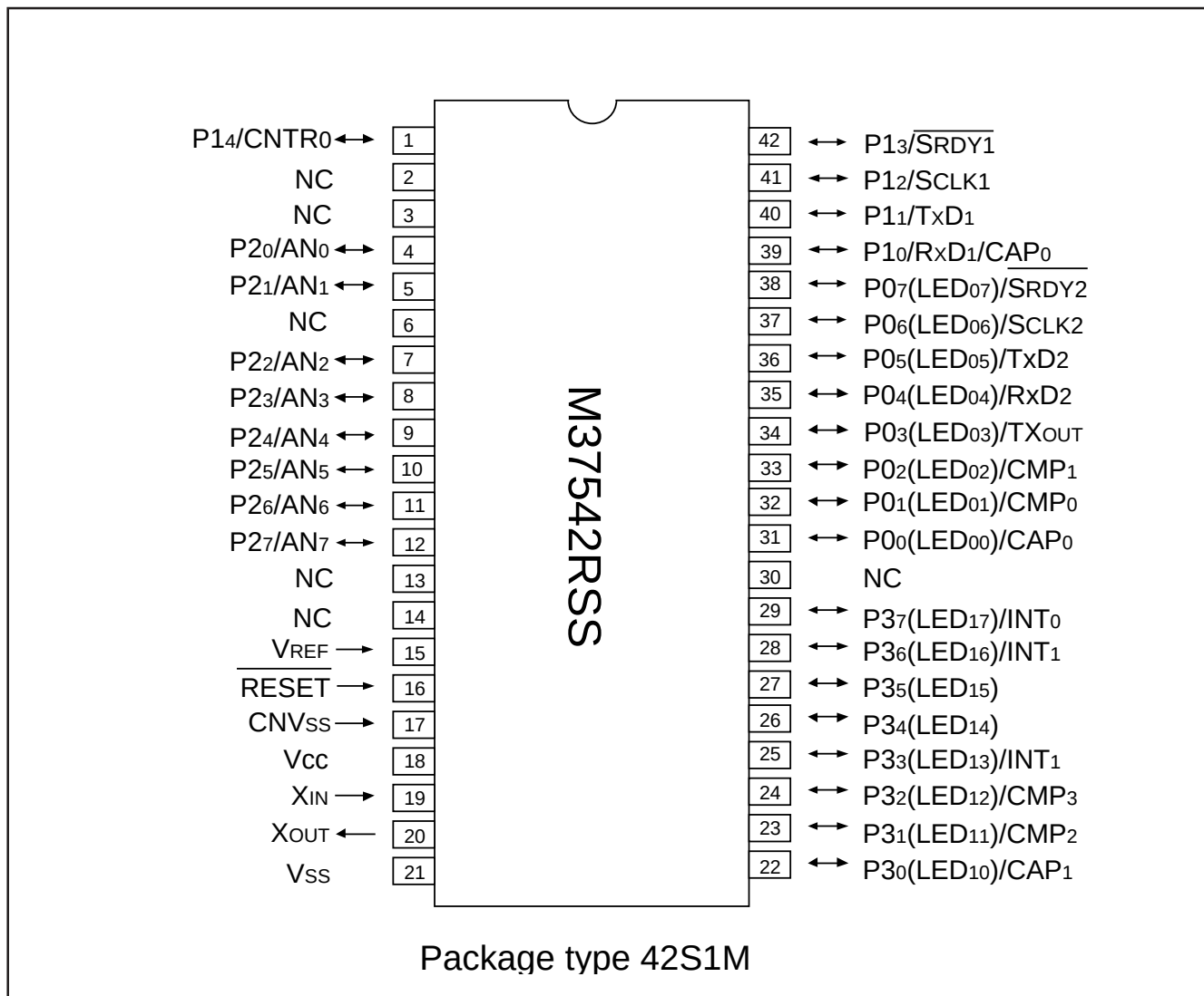
Fig. 5 Pin configuration (Package type: 42S1M)
