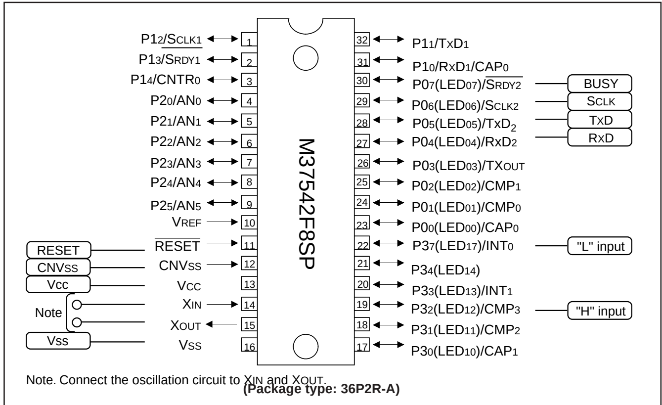
Fig. 105 Pin connection diagram in standard serial I/O mode 1 (36P2R-A package)
