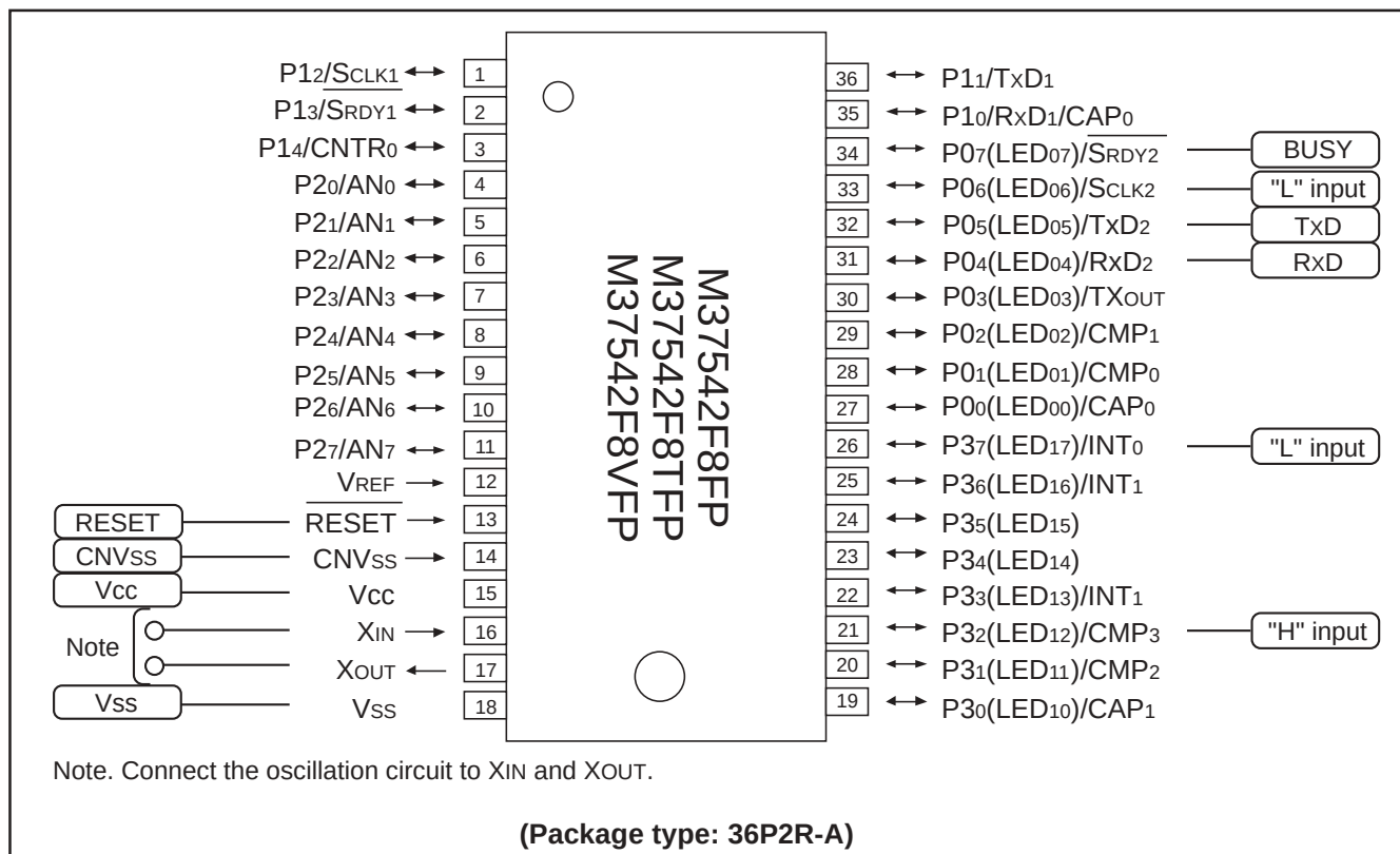
Fig. 110 Pin connection diagram in standard serial I/O mode 2 (36P2R-A package)
