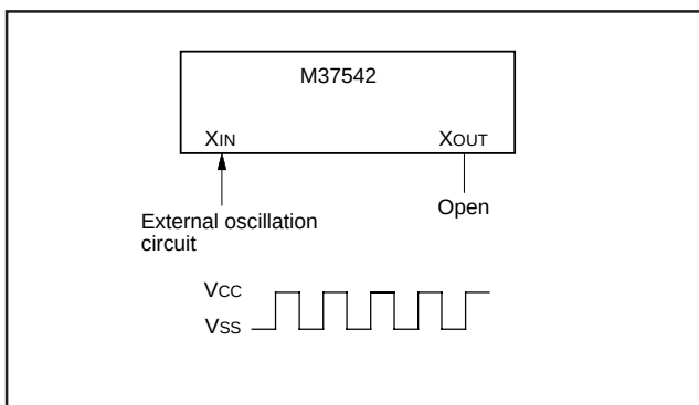
Fig. 76 External clock input circuit
