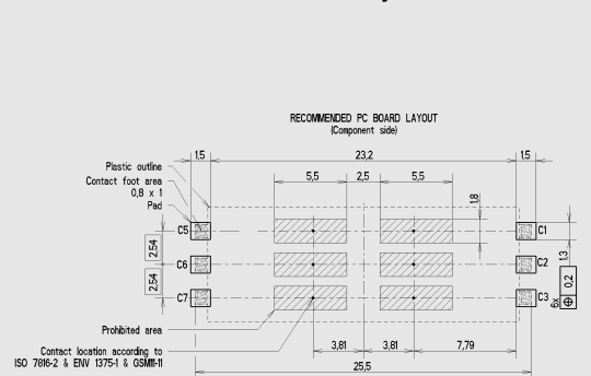
CCM04-1801 PCB Layout
