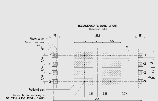
CCM04-1814 PCB layout
