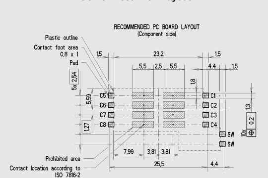
CCM04-1889 PCB Layout
