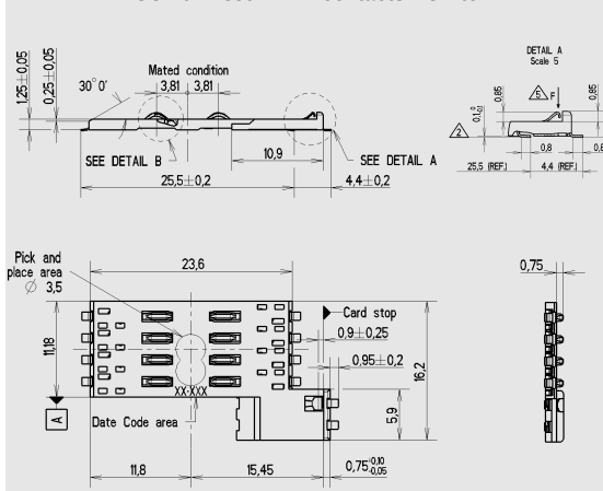
CCM04-1889 2 x 4 contacts + switch
