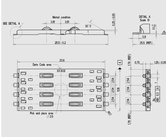
CCM04-1814 2 x 4 contacts
