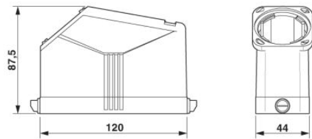
Dimensioned drawing
