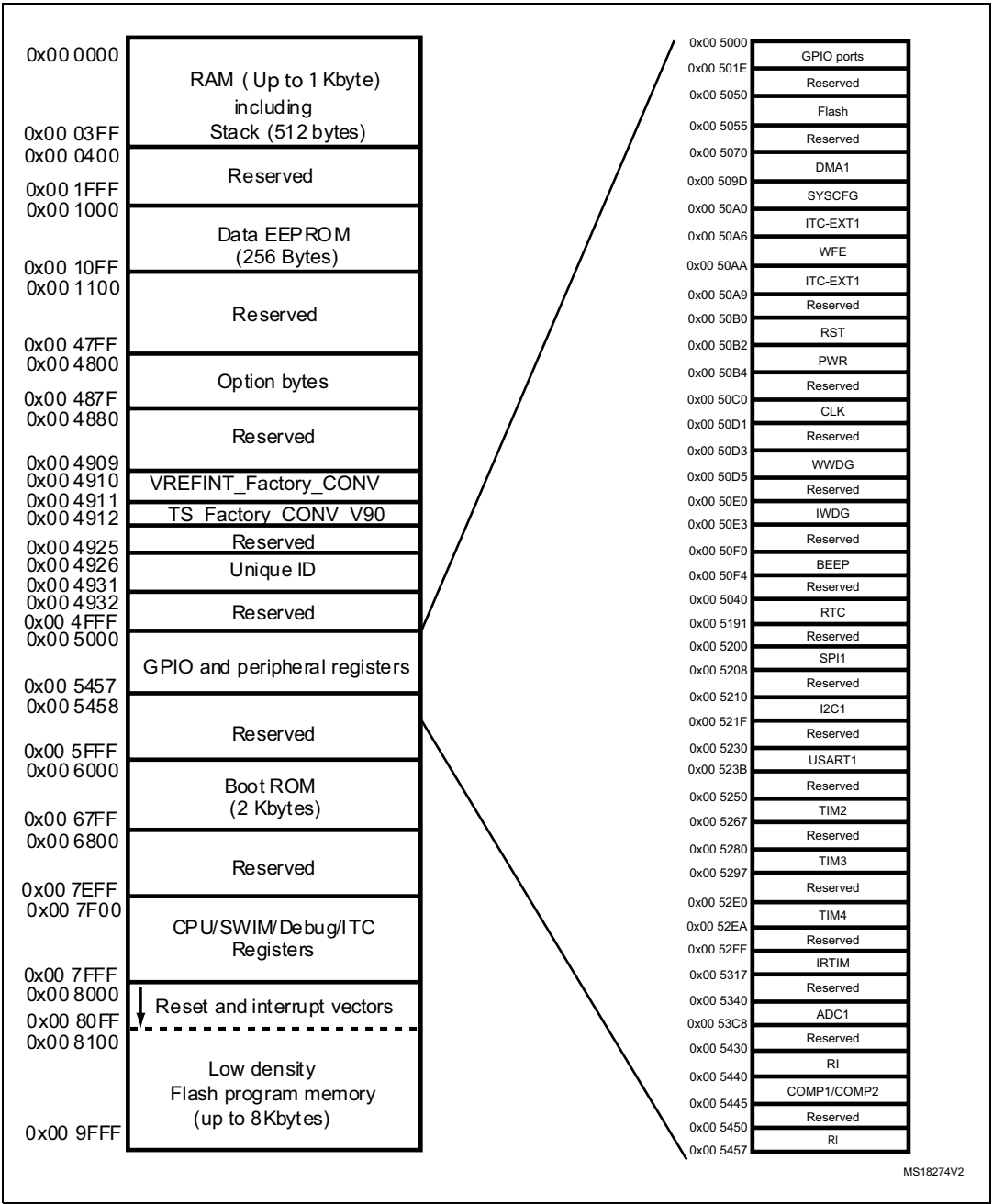
Figure 8. Memory map
