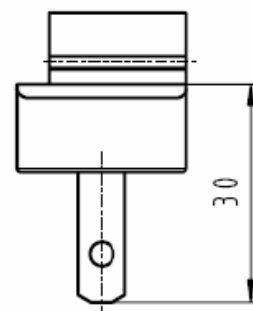
USA-Stecker/plug 1717715
