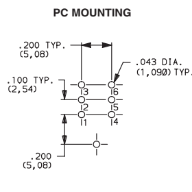
T201MH9AVBE Vertical Actuation DPDT
