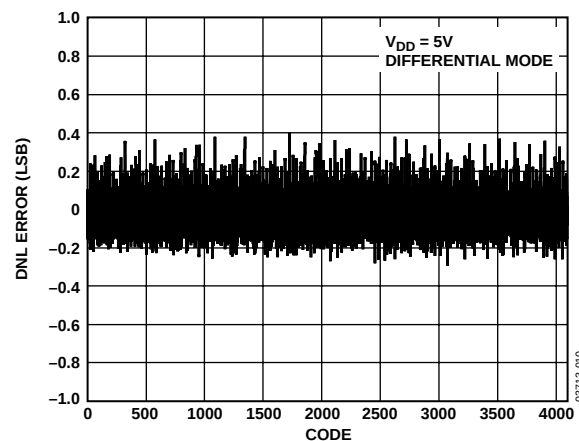
Figure 7. AD7934 Typical DNL @ V_{DD} = 5\text{ V}
