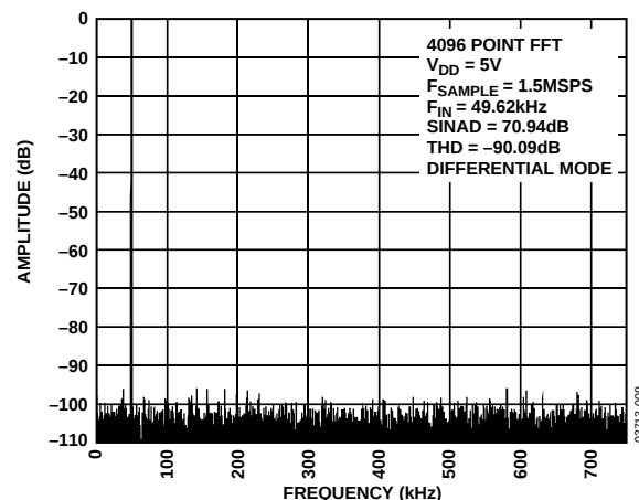
Figure 6. AD7934 FFT @ V_{DD} = 5\text{ V}
