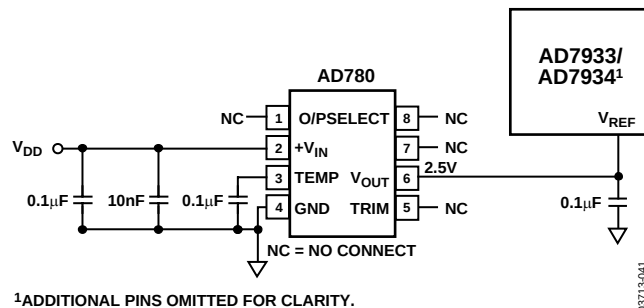
Figure 33. Typical V_{\text{REF}} Connection Diagram
