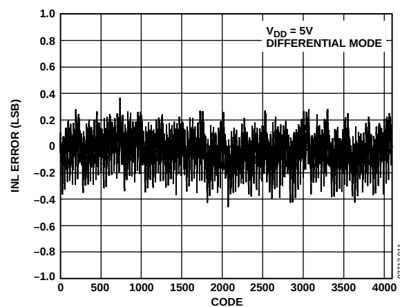
Figure 8. AD7934 Typical INL @ V_{DD} = 5\text{ V}
