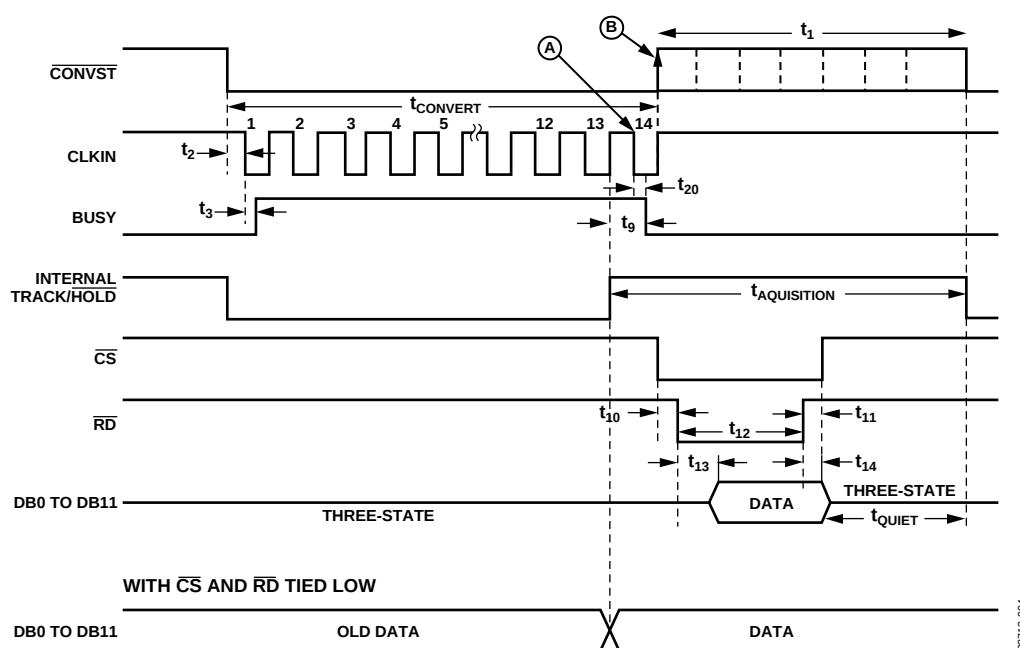
Figure 34. AD7933/AD7934 Parallel Interface—Conversion and Read Cycle in Word Mode ( \overline{W/B} = 1 )
