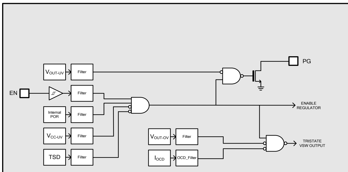
Figure 3: Monitor & Control Logic Functionality
