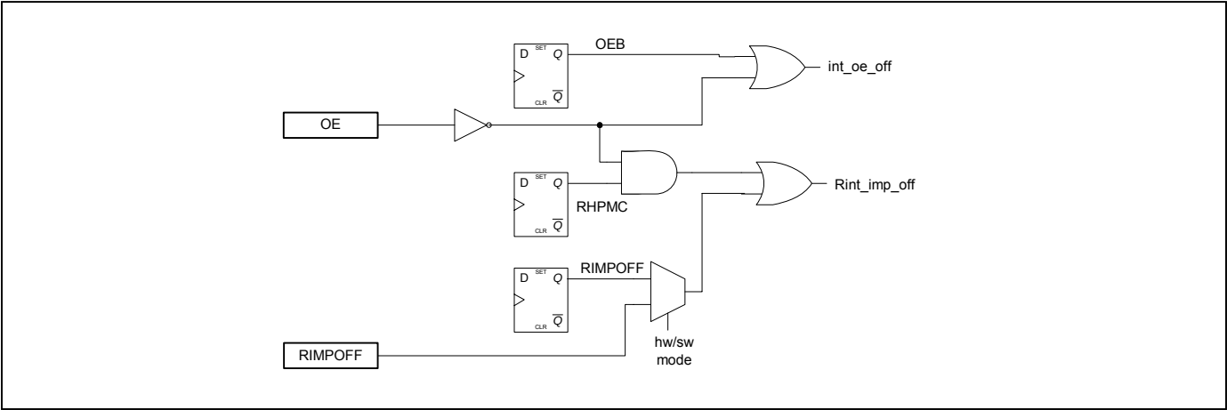
Figure 6-5. HPS Logic
