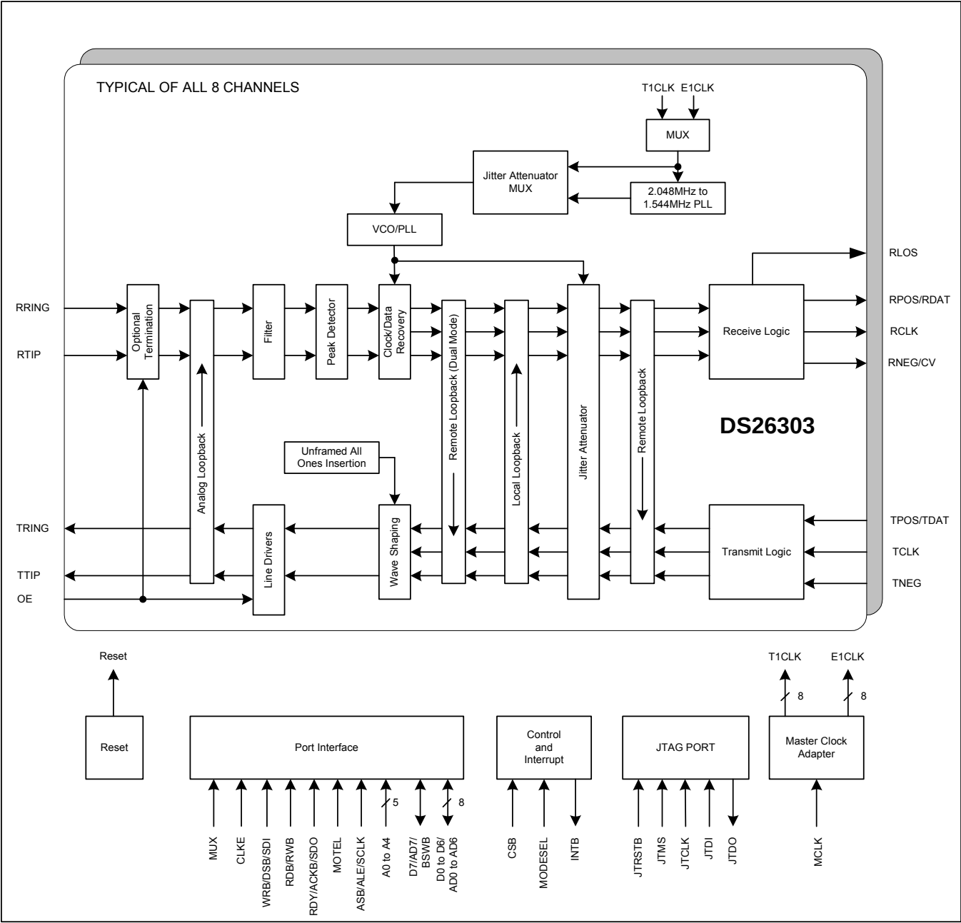
Figure 3-1. Block Diagram
