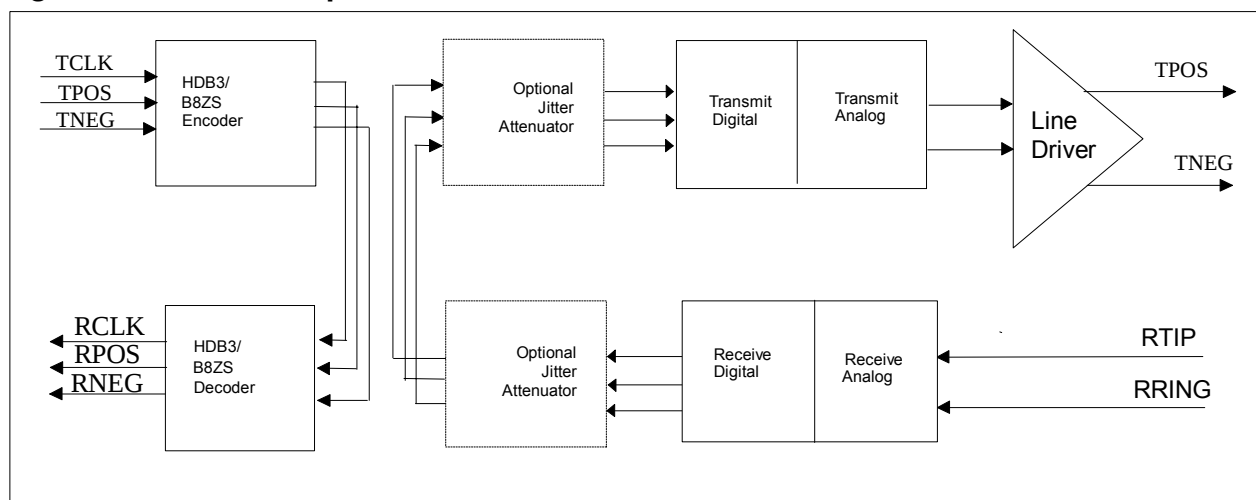
Figure 6-11. Dual Loopback
