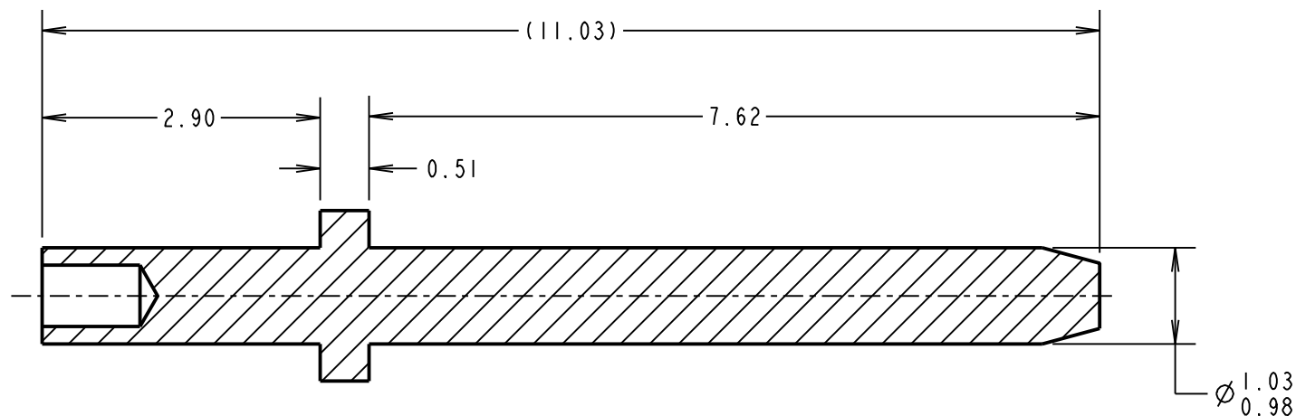
SECTION X-X
