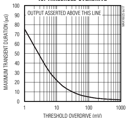
MAXIMUM TRANSIENT DURATION vs. THRESHOLD OVERDRIVE
