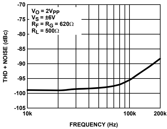
FIGURE 21. THD + NOISE vs FREQUENCY
