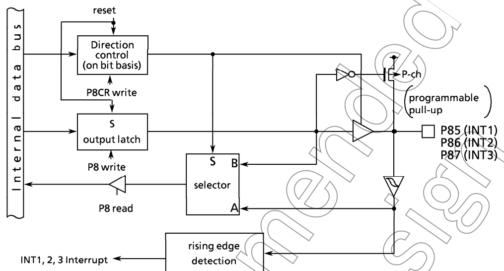
Figure 3.5 (14) Port 8: P85, P86, and P87
