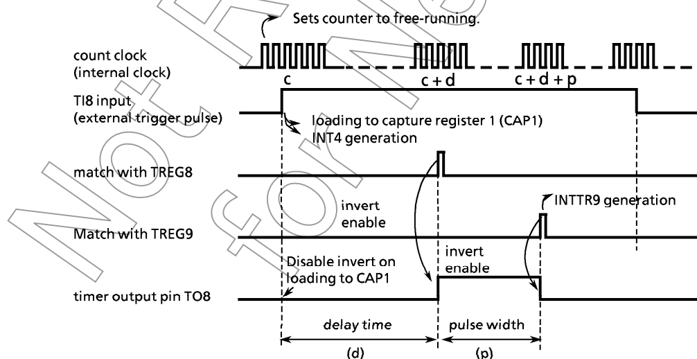
Figure 3.9 (13) One-Shot Pulse Output (With Delay)
