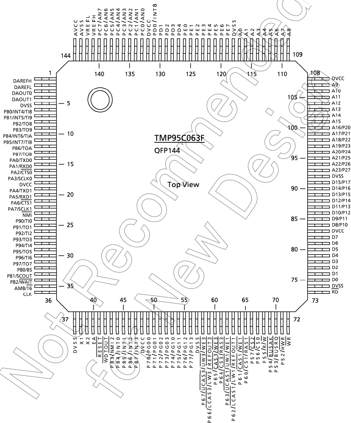
Figure 2.1 Pin Assignment
