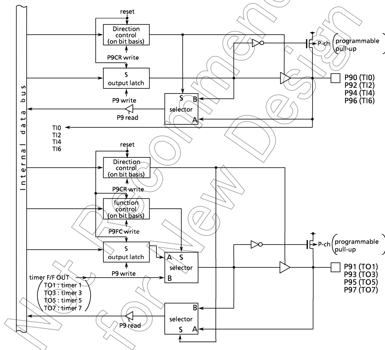
Figure 3.5 (16) Port 9
