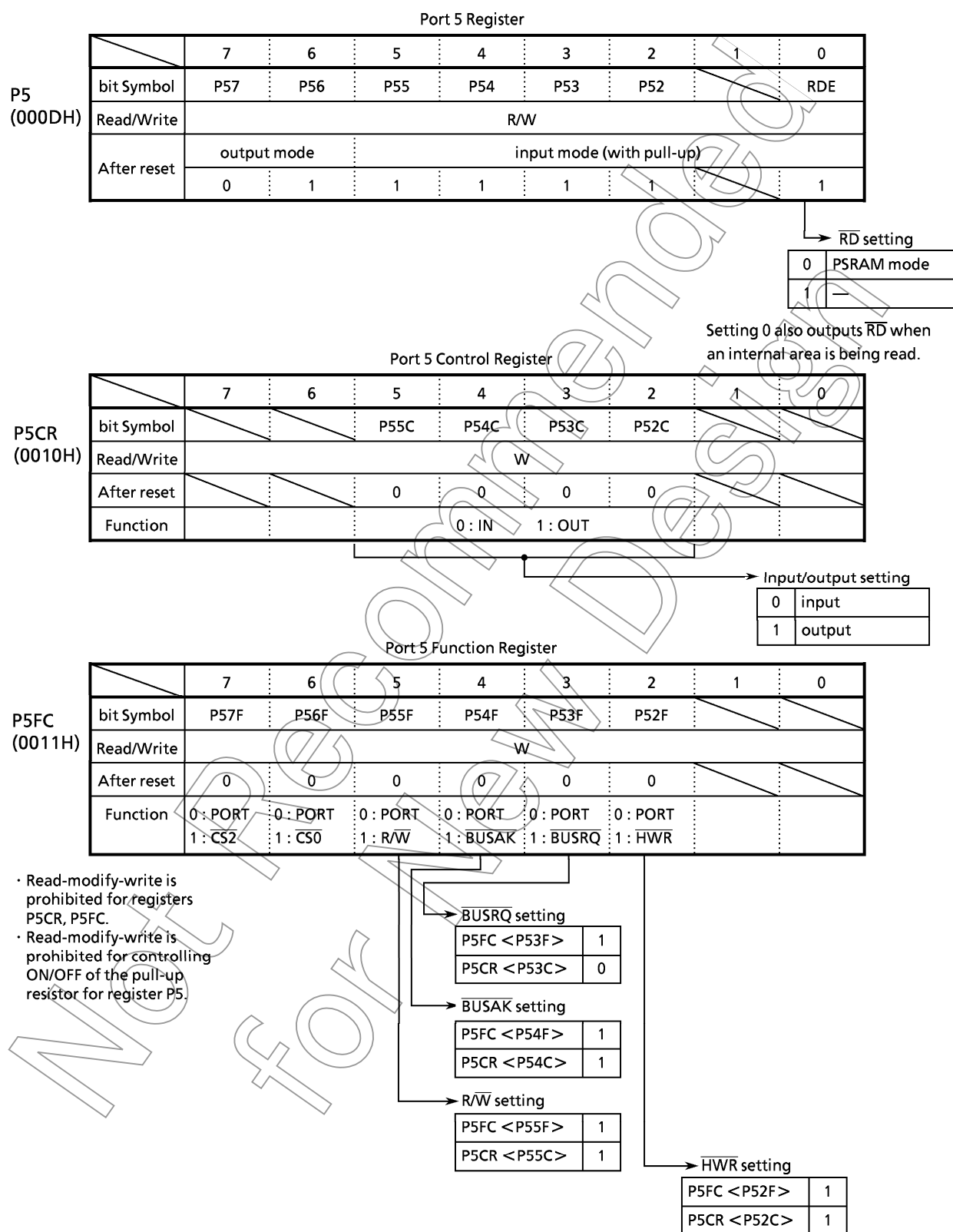
Figure 3.5 (7) Port 5 Registers
