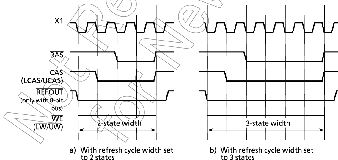
Figure 3.7 (5) Refresh Cycle Timing Examples
