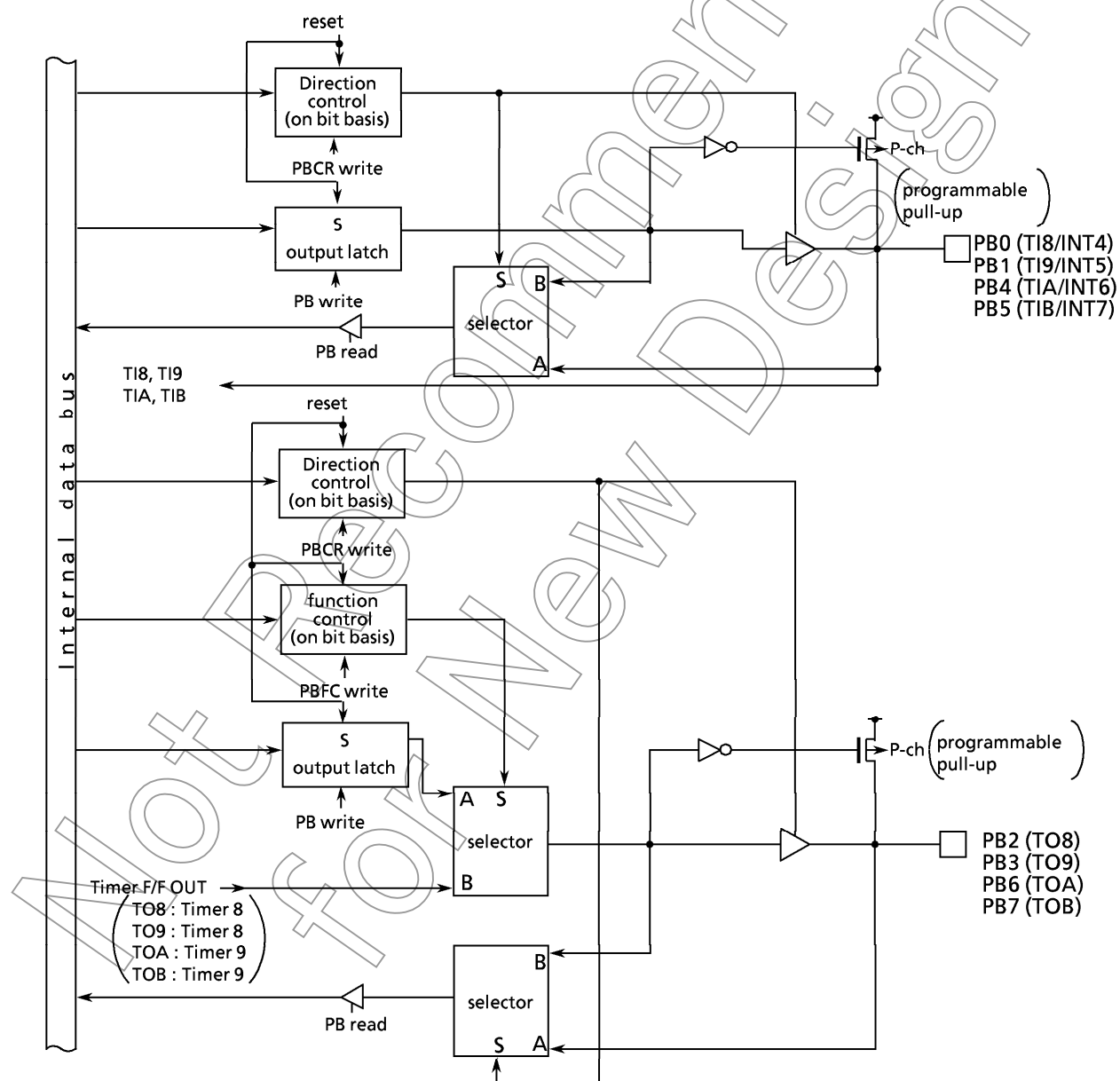
Figure 3.5 (23) Port B: PB0-PB7
