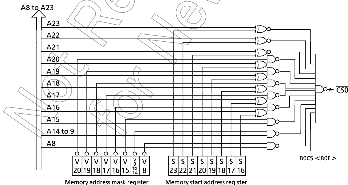
Figure 3.6 (5) \overline{CS0} Address Decoder Block Diagram
