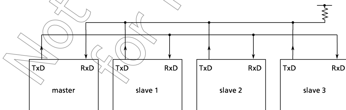
Figure 3.11 (22) Serial Link with Wake-Up Function
