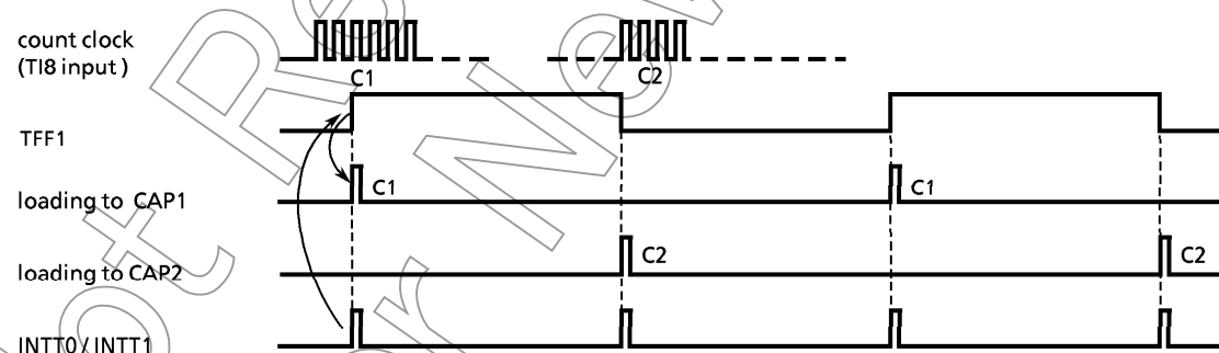
Figure 3.9 (15) Frequency Measurement
