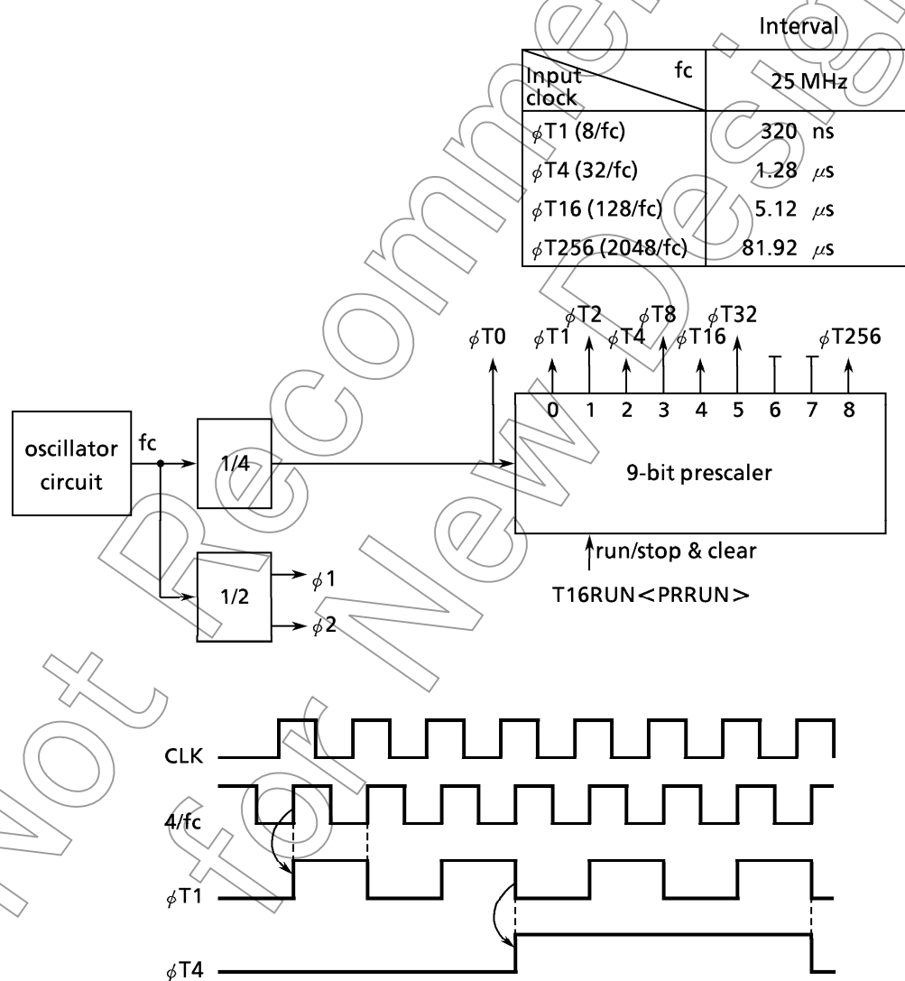
Figure 3.8 (2) Prescaler
