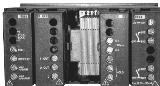
Rear View Assembled Unit
