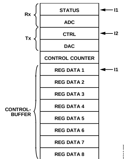
Figure 5. Buffer Memory Map
