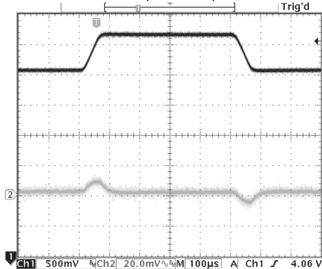
Line Transient (LDO1) 3.6 - 4.5 Vin, 3.3 Vout, 150 mA load
