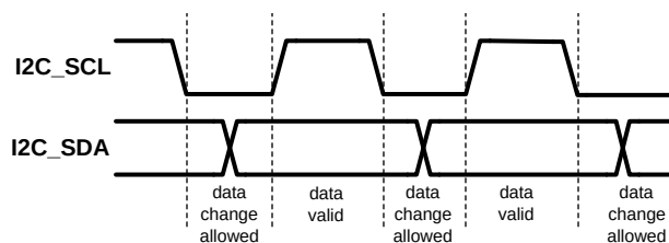
Figure 59. I 2 C Signals: Data Validity
