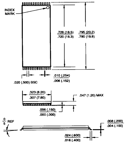
32T, 32 Lead, Thin Small Outline Package (TSOP) Dimensions in Inches and (Millimeters)
