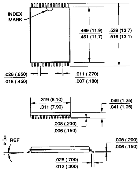
28T, 28 Lead, Thin Small Outline Package (TSOP) Dimensions in Inches and (Millimeters)
