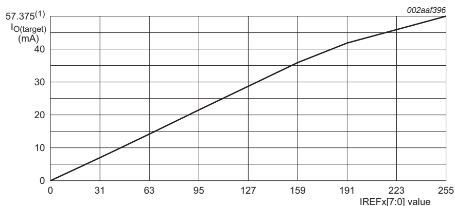
Fig 7. I_{\text{O(target)}} versus IREFx value
