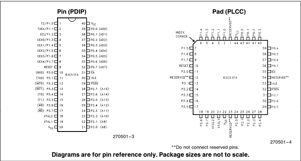
Figure 3. Pin Connections
