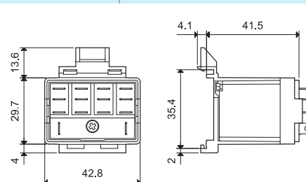
056.47 with relay
